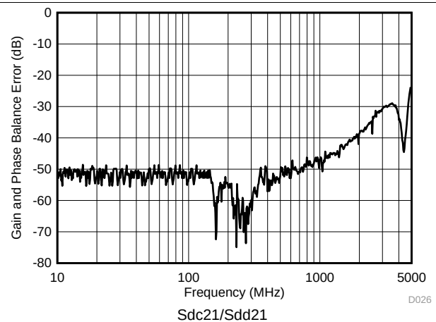
Figure 28. Output Balance Error vs Frequency
