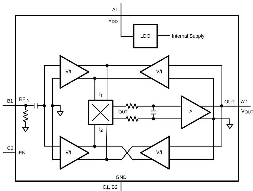
Figure 57. Block Diagram
