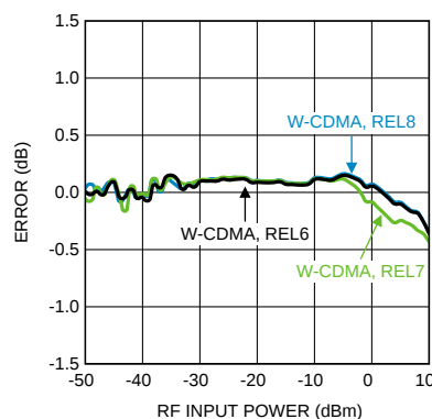
Figure 66. Variation due to Modulation for W-CDMA at 1900 MHz
