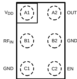
Figure 3. 6-Bump DSBGA Top View
