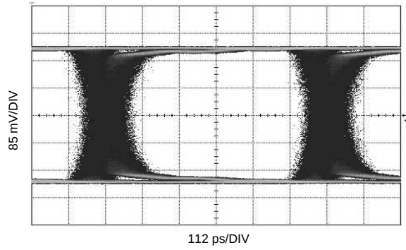
Figure 21. 1.485 Gbps, CC = 280 m Belden 1694A
