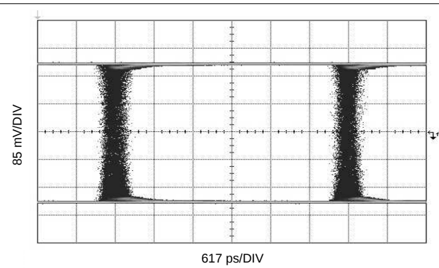
Figure 22. 270 Mbps, CC = 400 m Belden 1694A
