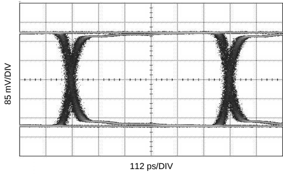
Figure 20. 1.485 Gbps, CC = 200 m Belden 1694A
