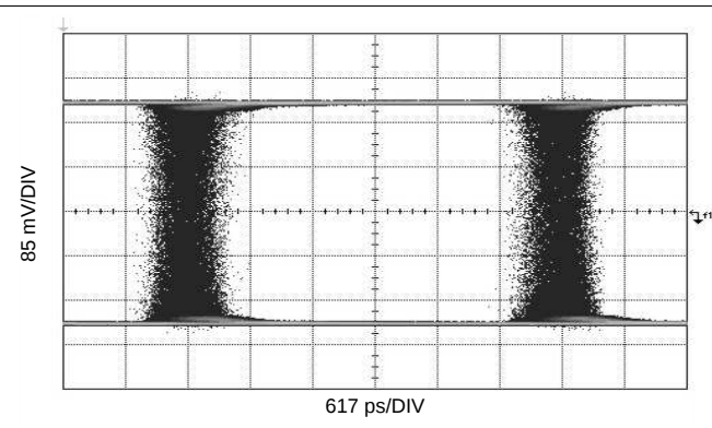
Figure 23. 270 Mbps, CC = 600 m Belden 1694A
