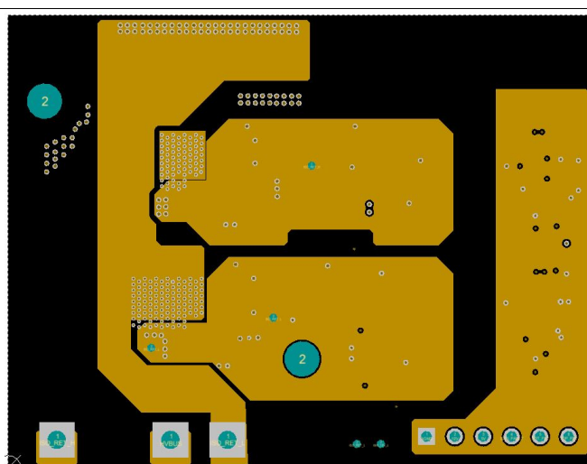
Figure 16. LMG341xEVM-018 Inner Copper Layer 1
