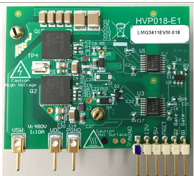
Figure 3. Back Side View of LMG341xEVM-018
