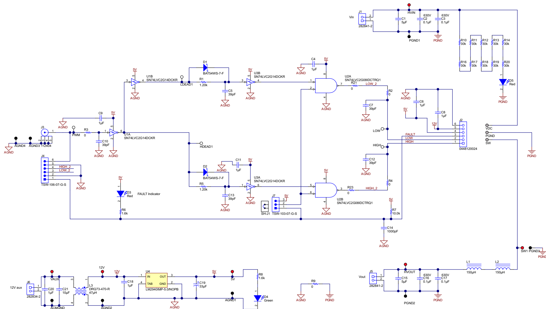
Figure 6. LMG34XX-BB-EVM Schematic
