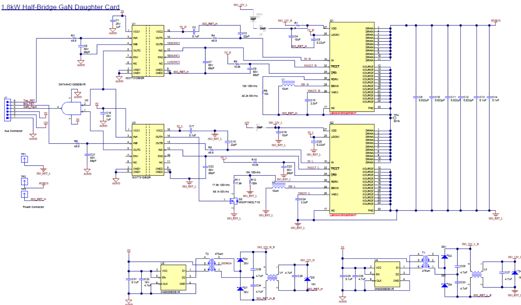
Figure 4. LMG3410EVM-018 Schematic
