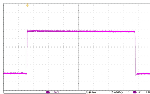
Figure 12. Switching Waveforms with 480V input, 100kHz, 30% duty cycle, 6A output
