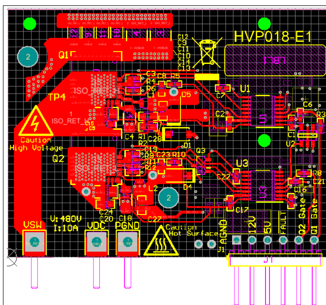
Figure 15. LMG341xEVM-018 Top Layer and Components
