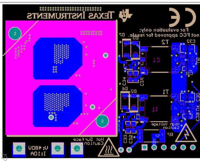
Figure 18. LMG341xEVM-018 Bottom Layer and Components
