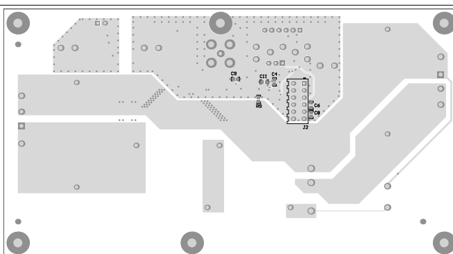
Figure 20. LMG34XX-BB-EVM Bottom Layer and Components
