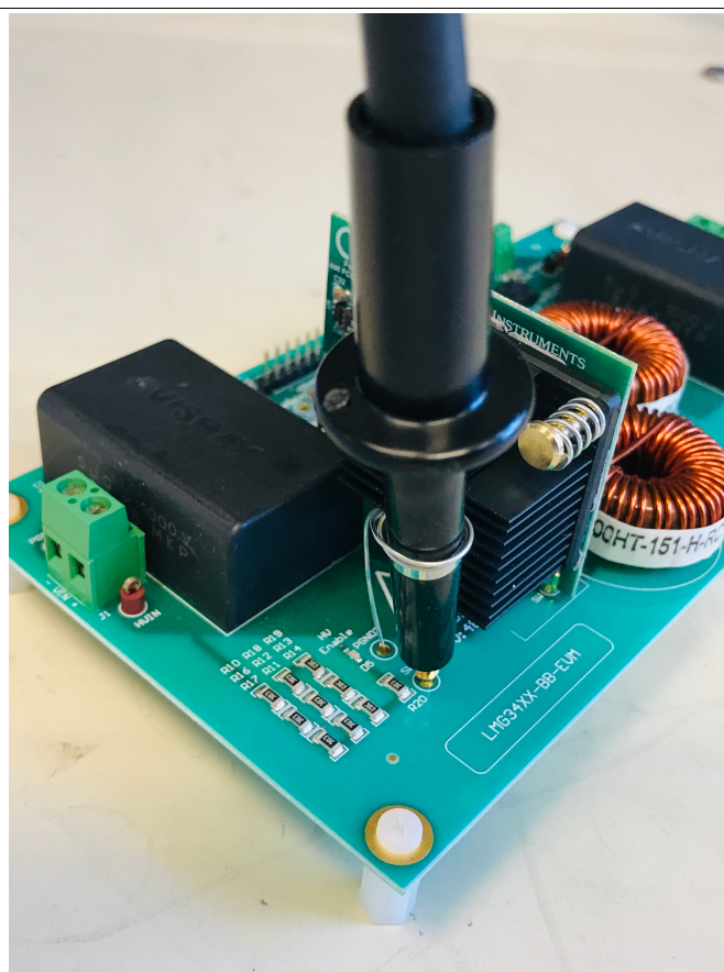
Figure 10. Recommended Probe Connection for High Voltage Switch Node
