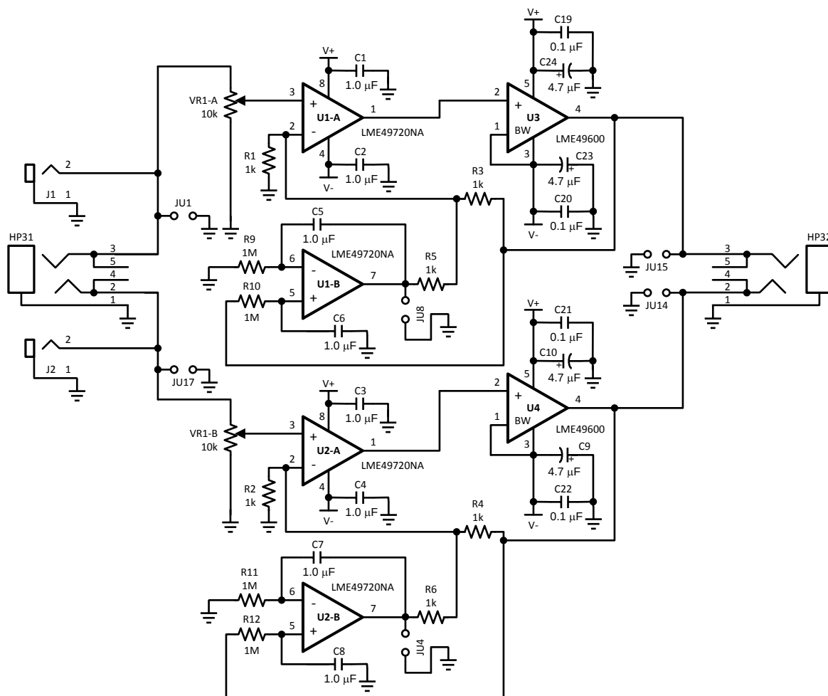
Figure 28. LME49600 Delivers High Output Current for this High Performance Headphone Amplifier
