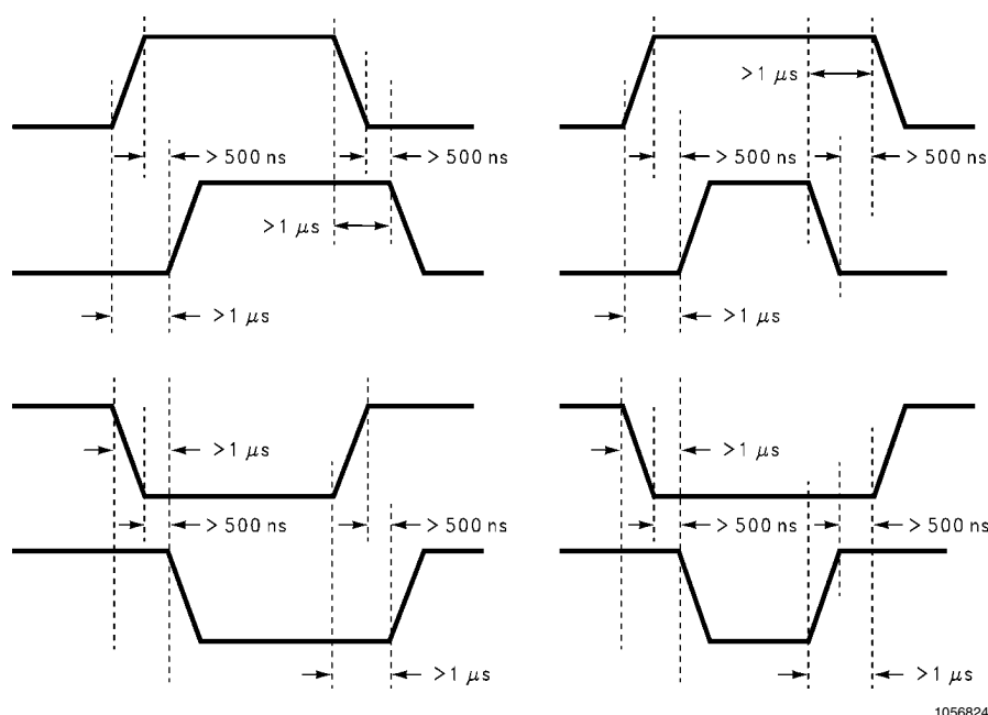
FIGURE 4. Transitions in Brake, Direction, or PWM Must Be Separated By At Least 1 \mu s
