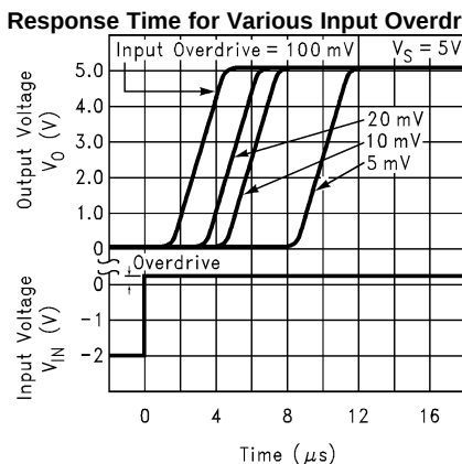
Response Time for Various Input Overdrives -t_{PLH}
