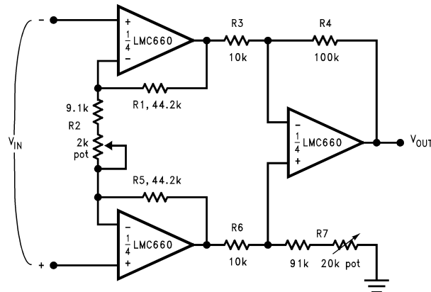
Figure 24. Instrumentation Amplifier
