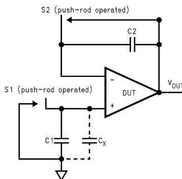
Figure 22. Simple Input Bias Current Test Circuit
