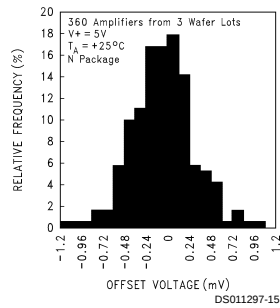
Distribution of LMC6082 Input Offset Voltage ( T_A = +25^\circ C )
