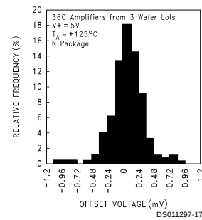
Distribution of LMC6082 Input Offset Voltage ( T_A = +125^\circ C )
