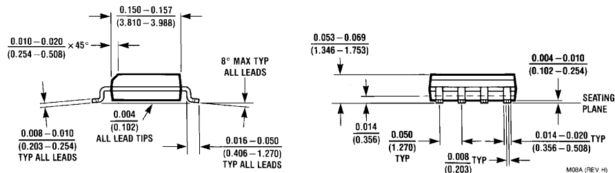
8-Pin Small Outline Package Order Number LMC6082AIM or LMC6082IM NS Package Number M08A
