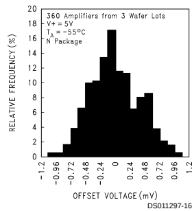
Distribution of LMC6082 Input Offset Voltage ( T_A = -55^\circ C )
