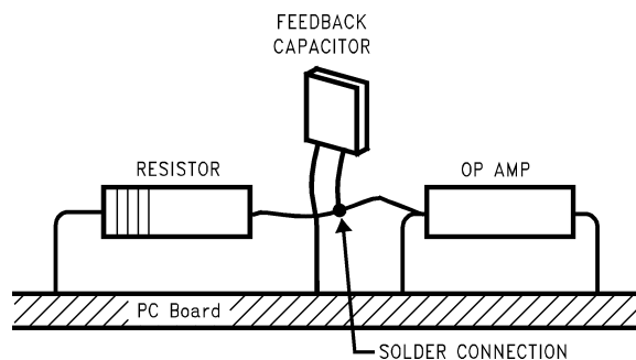
Figure 34. Air Wiring
