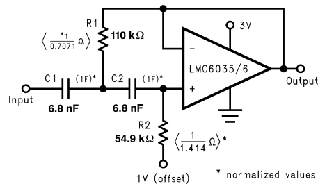
Figure 48. 2 Pole, 300Hz, Sallen and Key, High-Pass Filter
