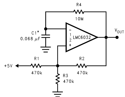
Figure 29. 1 Hz Square-Wave Oscillator
