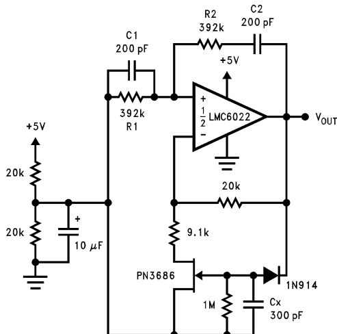
Figure 36. Instrumentation Amplifier
