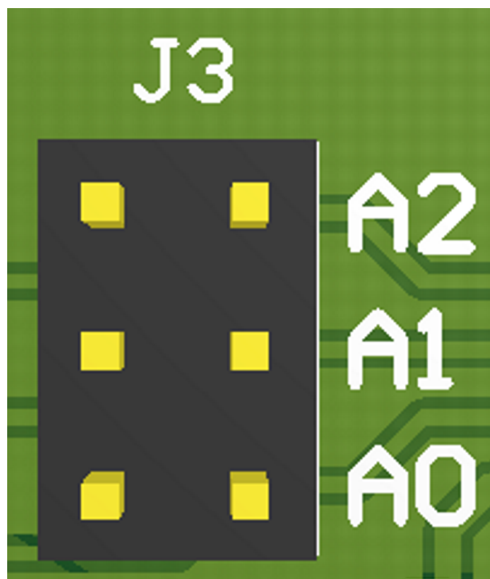
Figure 2-5. I²C Slave Select Jumper
