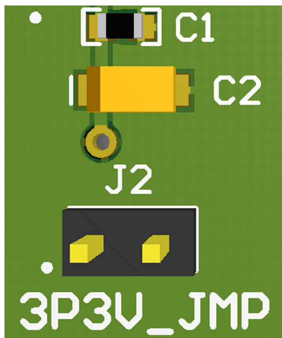
Figure 2-2. VCC Jumper
