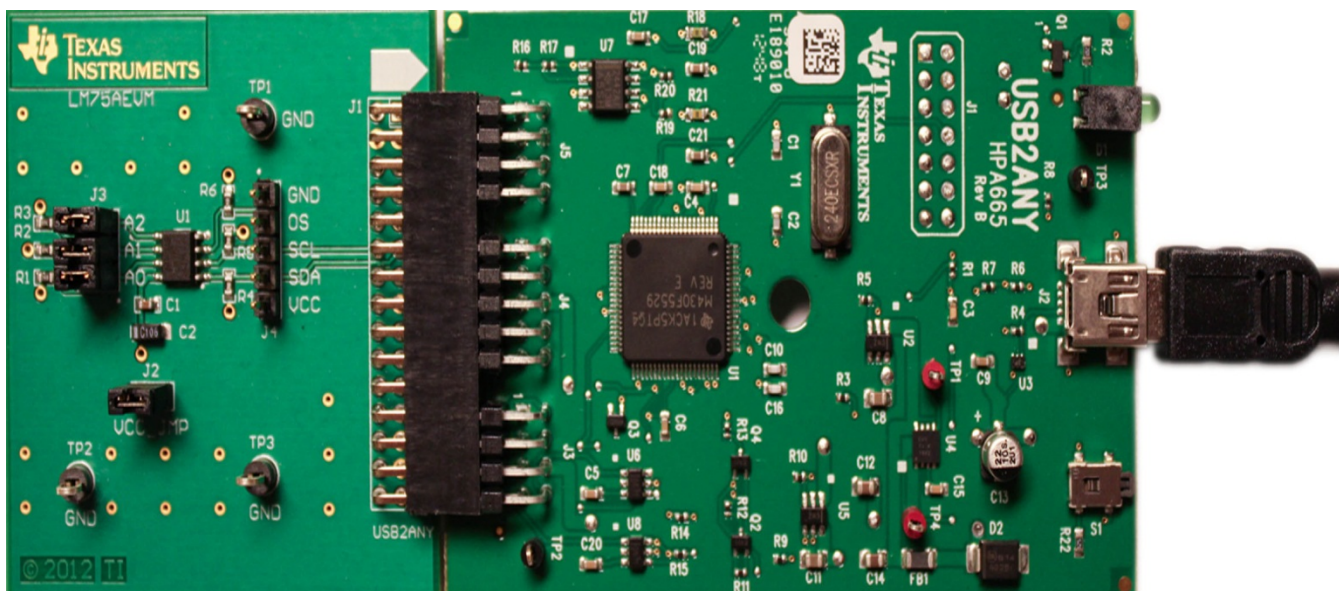
Figure 4-1. LM75AEVM Hardware Connection
