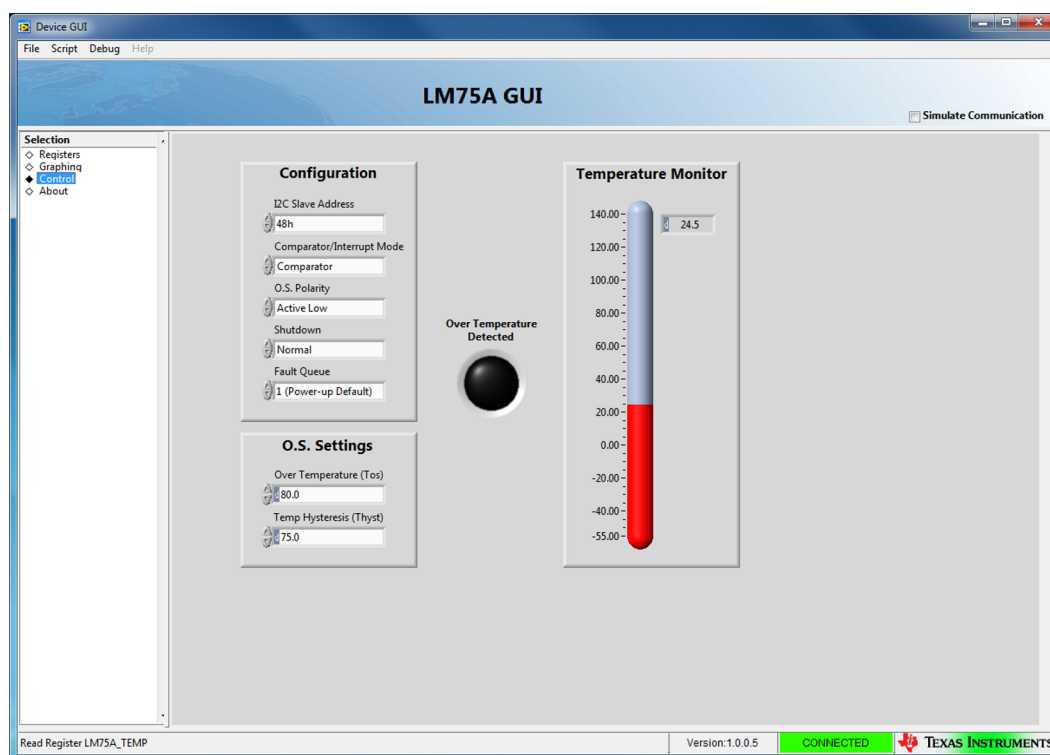
Figure 4-4. Control Tab
