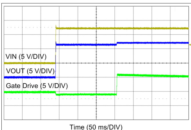
Figure 14. Startup Relative to V_{IN}
