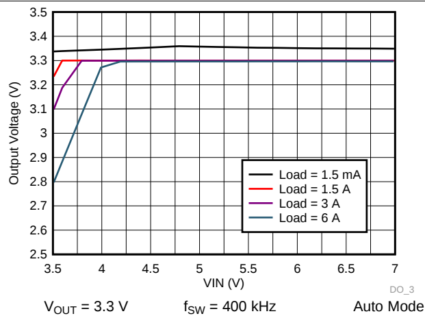
Figure 65. LM73606-Q1 Dropout Curve
