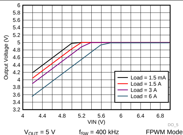
Figure 60. LM73606-Q1 Dropout Curve
