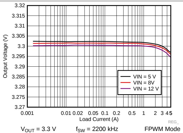
Figure 54. LM73605-Q1 Load and Line Regulation
