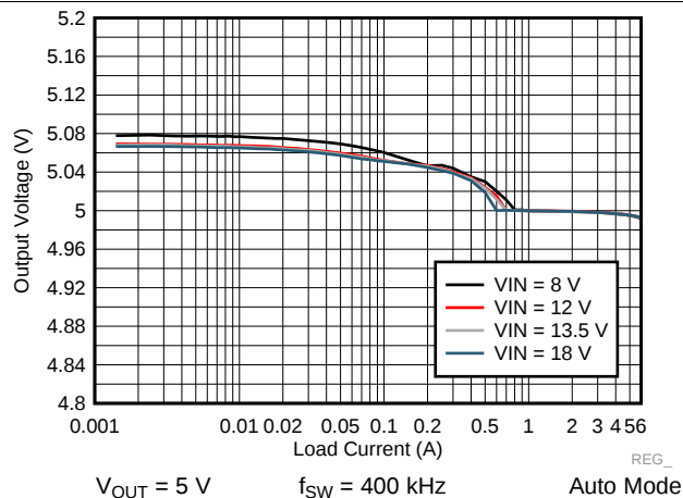
Figure 45. LM73606-Q1 Load and Line Regulation
