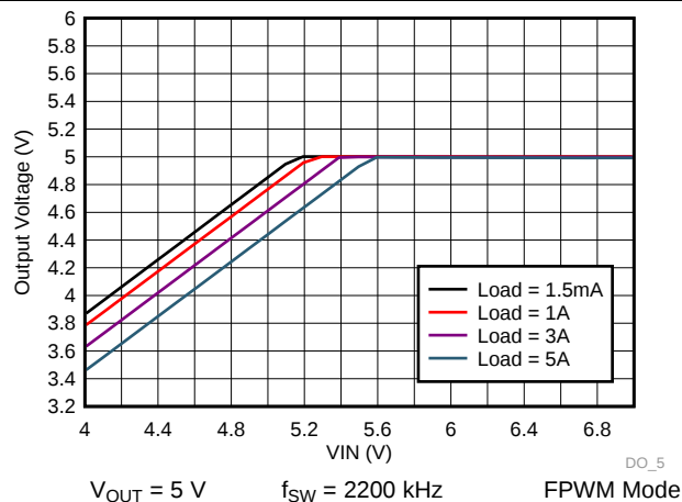
Figure 62. LM73605-Q1 Dropout Curve
