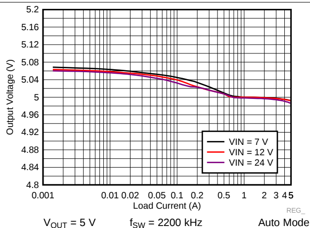
Figure 49. LM73605-Q1 Load and Line Regulation
