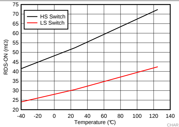
Figure 1. High-Side and Low-Side Switches R_{DS-ON}
