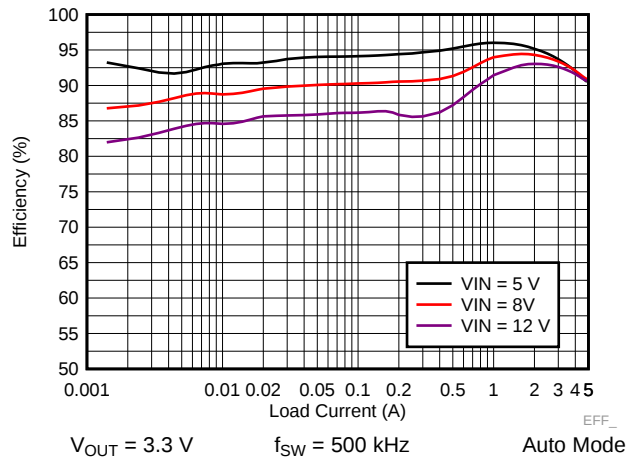
Figure 29. LM73605-Q1 Efficiency
