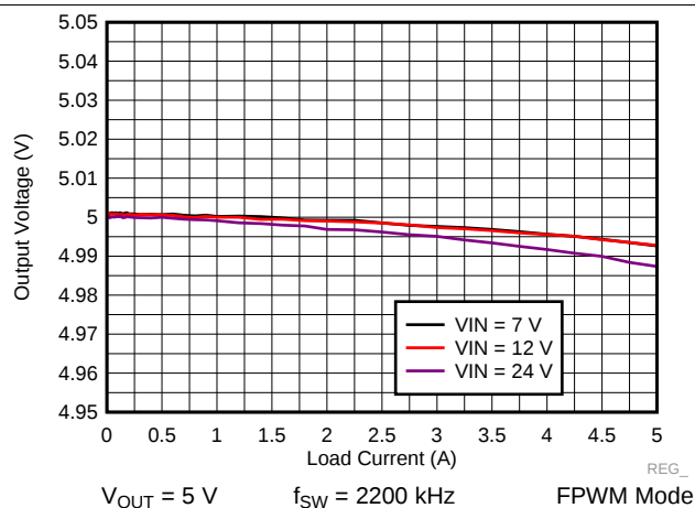
Figure 50. LM73605-Q1 Load and Line Regulation
