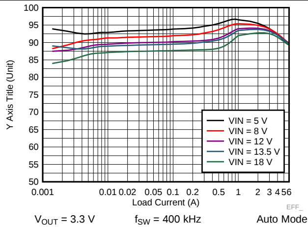
Figure 27. LM73606-Q1 Efficiency
