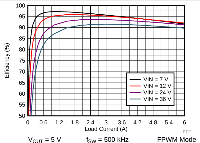
Figure 38. LM73606-Q1 Efficiency
