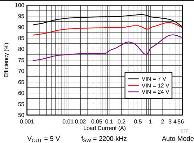
Figure 41. LM73606-Q1 Efficiency
