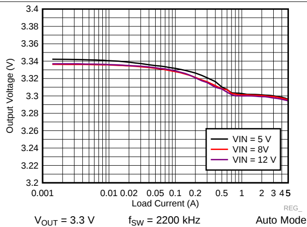
Figure 53. LM73605-Q1 Load and Line Regulation
