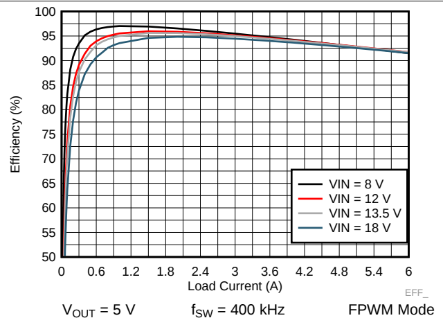
Figure 36. LM73606-Q1 Efficiency
