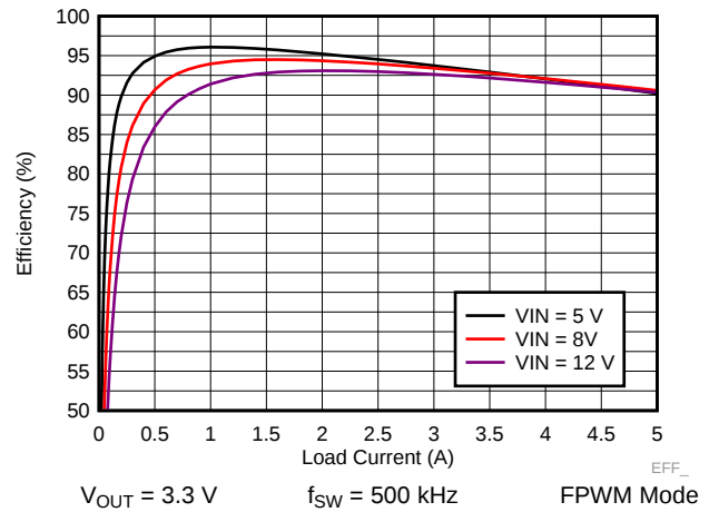
Figure 30. LM73605-Q1 Efficiency
