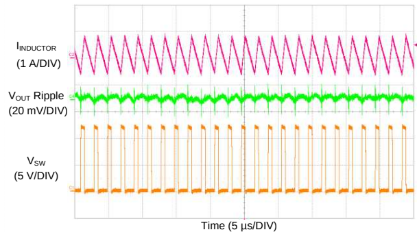
Figure 70. LM73606-Q1 Switching Waveform and V_{OUT} Ripple
