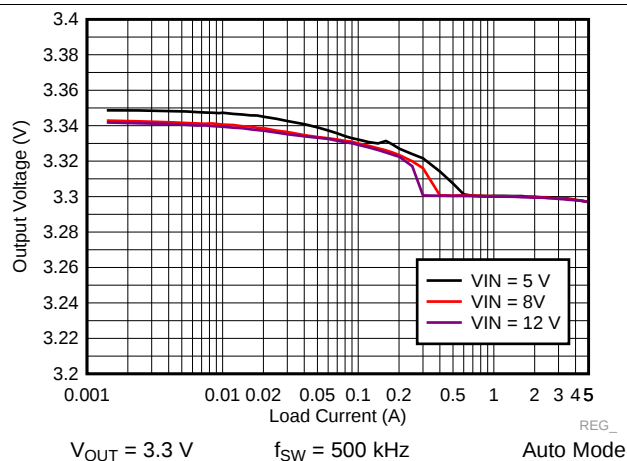
Figure 55. LM73605-Q1 Load and Line Regulation
