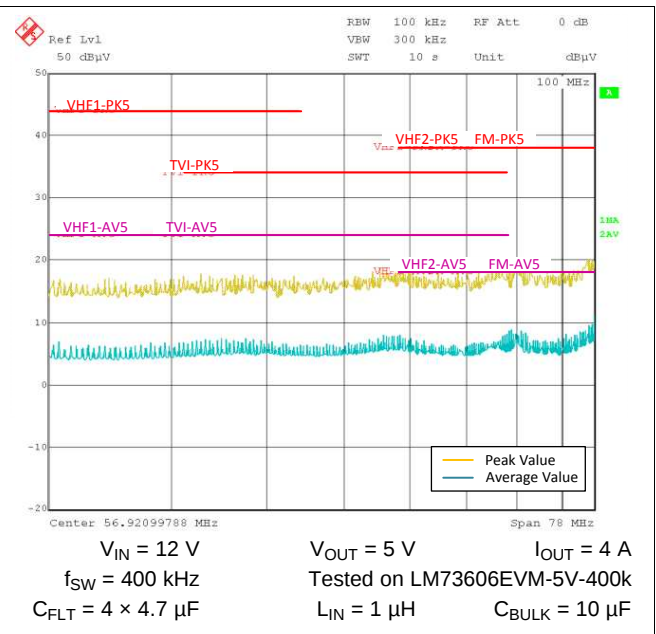
Figure 88. LM73606-Q1 Conducted EMI Result vs. CISPR25 Limits - High Frequency
