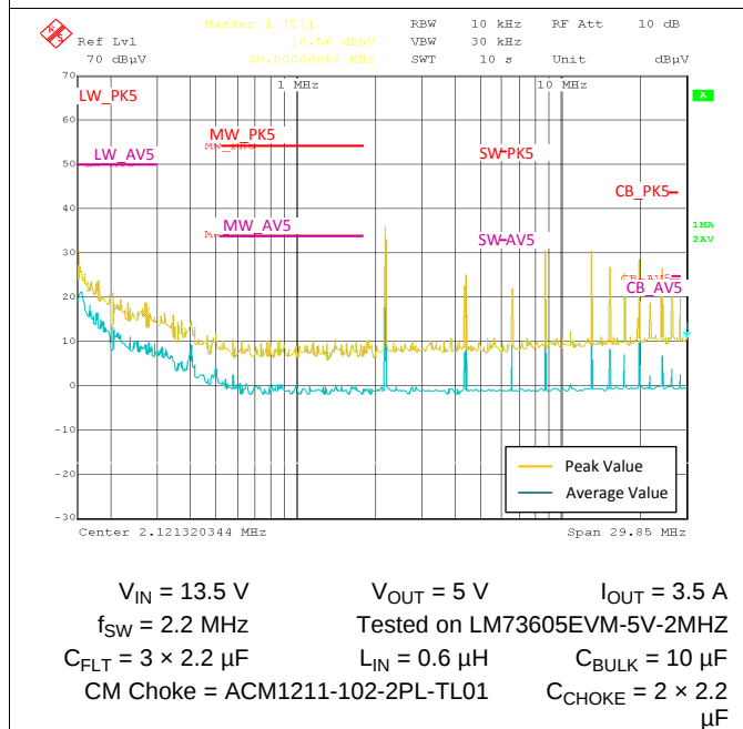
Figure 89. LM73606-Q1 Conducted EMI Result vs. CISPR25 Limits - Low Frequency
