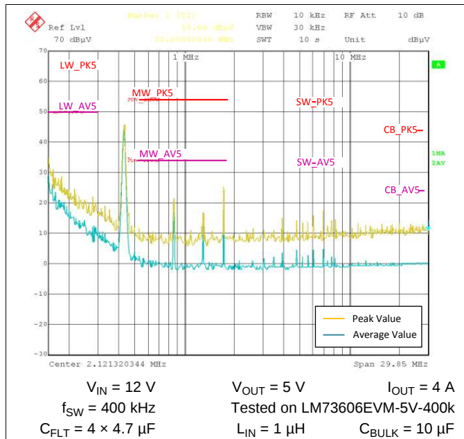
Figure 87. LM73606-Q1 Conducted EMI Result vs. CISPR25 Limits - Low Frequency
