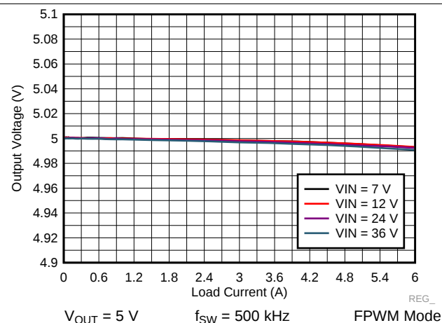
Figure 48. LM73606-Q1 Load and Line Regulation
