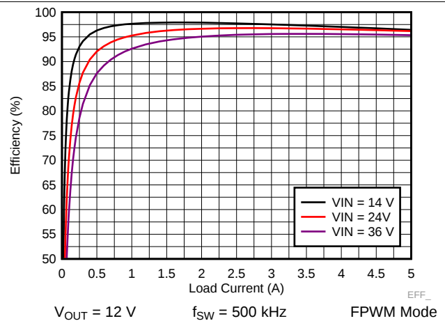
Figure 44. LM73605-Q1 Efficiency
