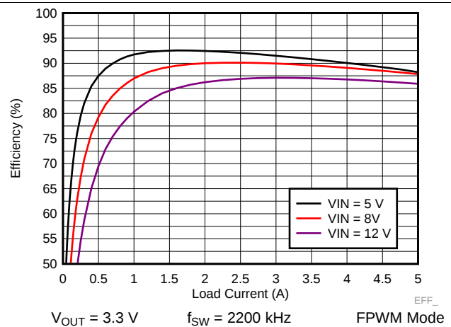
Figure 32. LM73605-Q1 Efficiency
