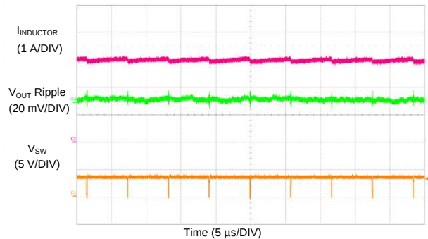
Figure 72. LM73606-Q1 Switching Waveform and V_{OUT} Ripple
