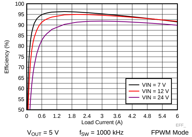
Figure 40. LM73606-Q1 Efficiency
