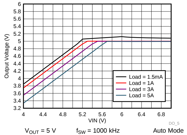
Figure 64. LM73605-Q1 Dropout Curve
