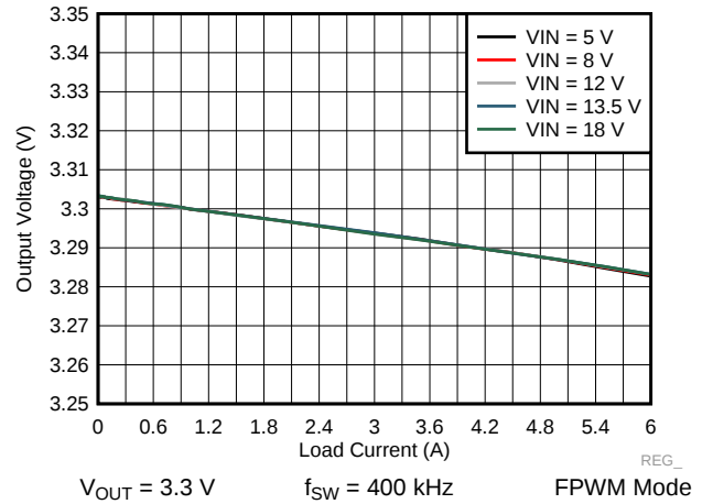
Figure 52. LM73606-Q1 Load and Line Regulation
