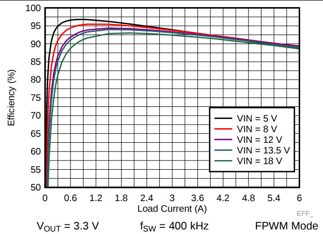
Figure 28. LM73606-Q1 Efficiency
