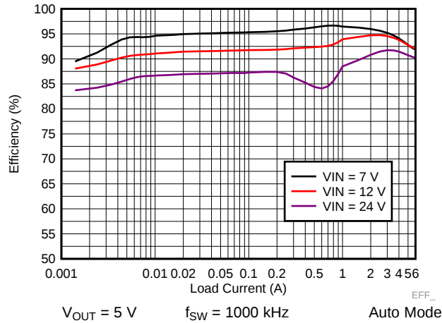
Figure 39. LM73606-Q1 Efficiency
