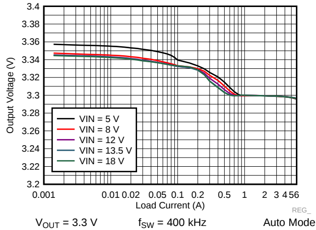
Figure 51. LM73606-Q1 Load and Line Regulation
