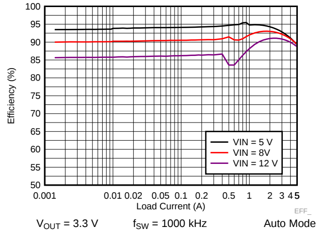
Figure 34. LM73605-Q1 Efficiency
