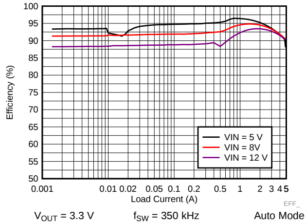
Figure 33. LM73605-Q1 Efficiency
