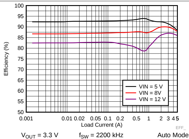
Figure 31. LM73605-Q1 Efficiency
