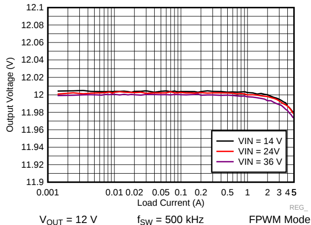
Figure 58. LM73605-Q1 Load and Line Regulation
