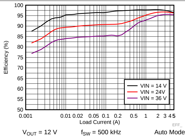
Figure 43. LM73605-Q1 Efficiency
