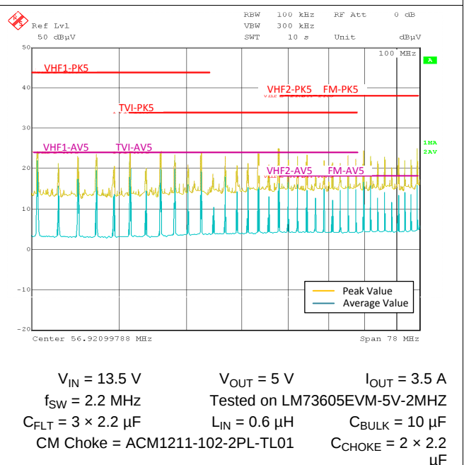
Figure 90. LM73606-Q1 Conducted EMI Result vs. CISPR25 Limits - High Frequency
