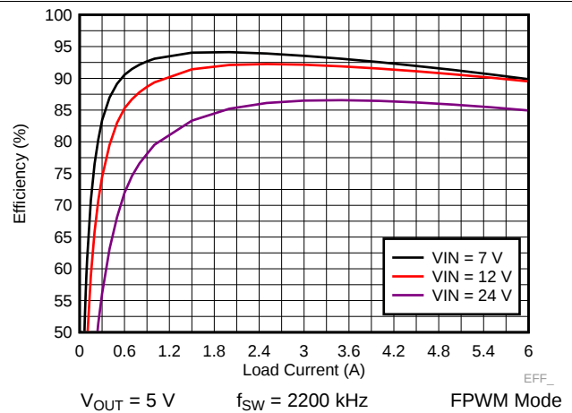
Figure 42. LM73606-Q1 Efficiency
