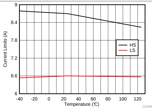
Figure 5. LM73605-Q1 High-Side and Low-Side Current Limit
