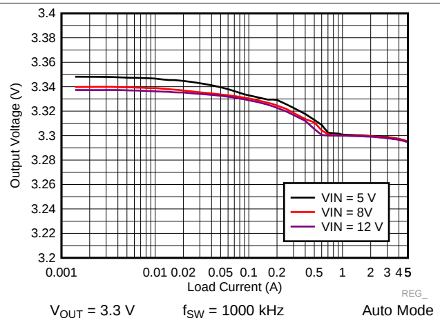
Figure 56. LM73605-Q1 Load and Line Regulation
