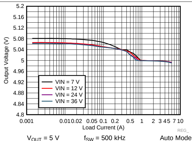
Figure 47. LM73606-Q1 Load and Line Regulation
