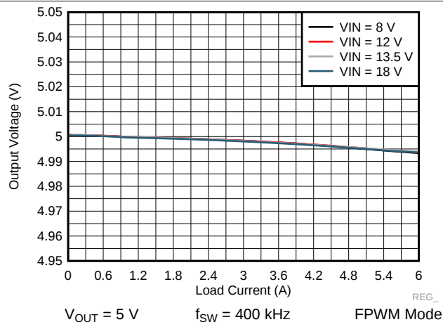
Figure 46. LM73606-Q1 Load and Line Regulation
