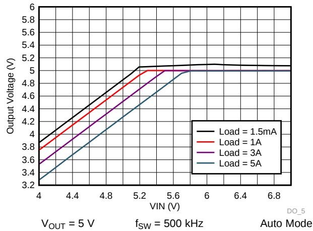
Figure 63. LM73605-Q1 Dropout Curve
