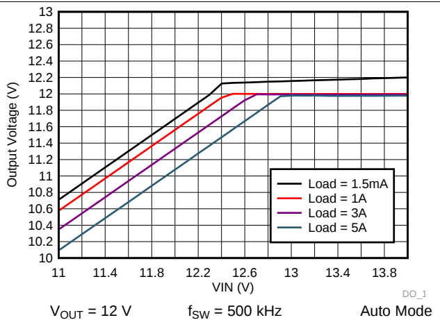
Figure 68. LM73605-Q1 Dropout Curve
