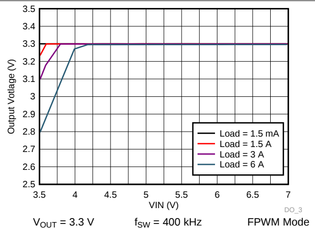
Figure 66. LM73606-Q1 Dropout Curve
