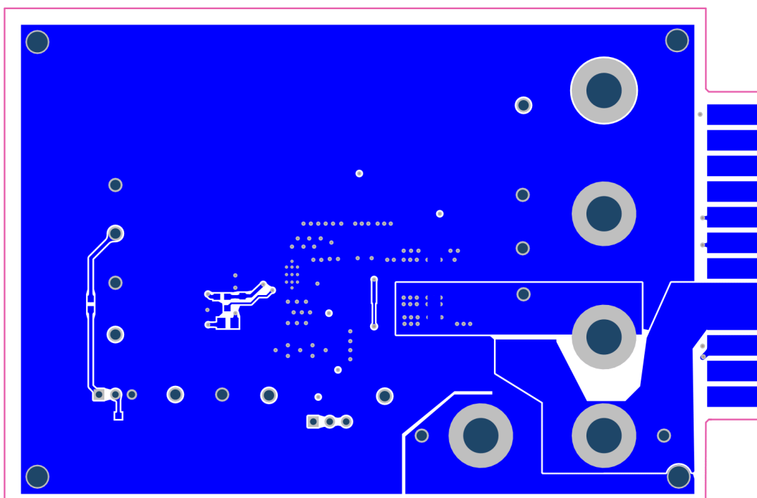
Figure 9. Bottom Layer Routing
