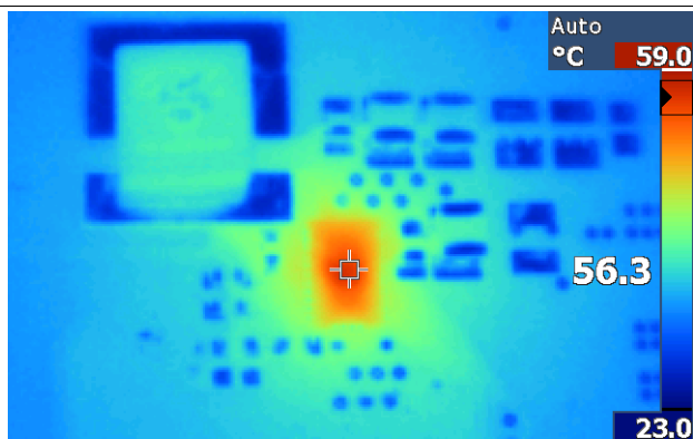
Figure 15. LM73605 5-V 2.2-MHz EVM Thermal Picture with V_{IN} = 12\text{ V} I_{OUT} = 5\text{ A}
