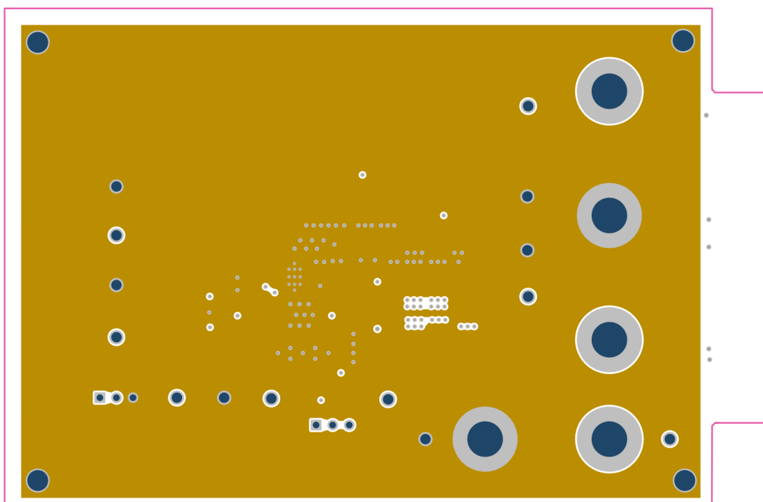
Figure 7. Mid-Layer 1 Ground Plane
