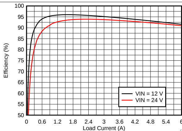
Figure 23. LM73606 5-V 400-kHz Efficiency in FPWM Mode
