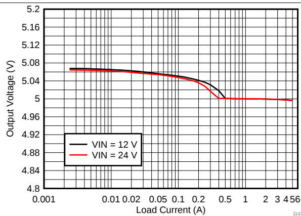
Figure 18. LM73605 5-V 400-kHz V_{OUT} Regulation in Auto Mode
