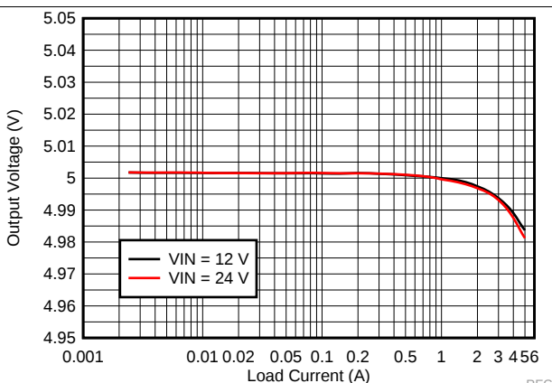
Figure 13. LM73605 5-V 2.2-MHz V_{OUT} Regulation in FPWM Mode
