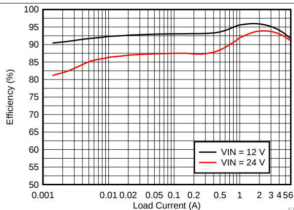
Figure 22. LM73606 5-V 400-kHz Efficiency in Auto Mode
