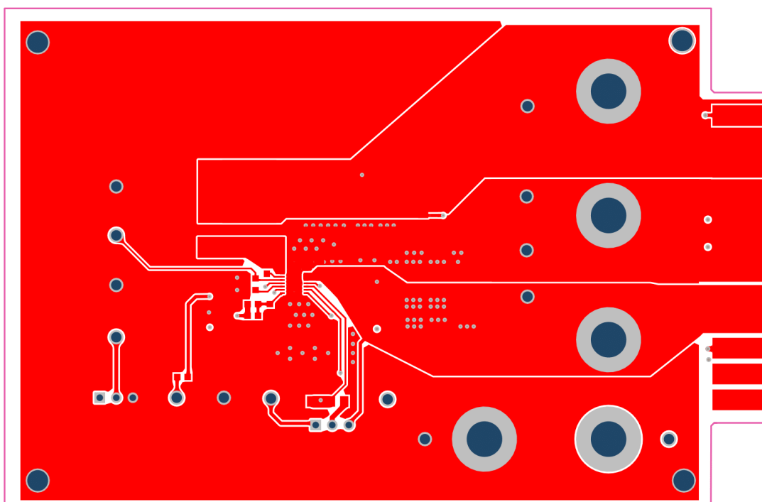
Figure 6. Top Layer Routing
