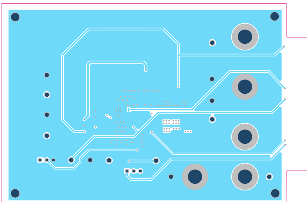
Figure 8. Mid-Layer 2 Routing
