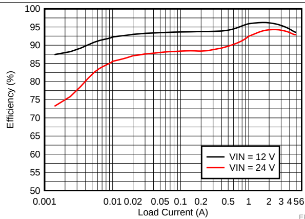
Figure 16. LM73605 5-V 400-kHz Efficiency in Auto Mode
