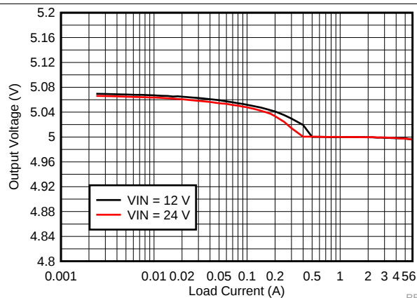
Figure 24. LM73606 5-V 400-kHz V_{OUT} Regulation in Auto Mode
