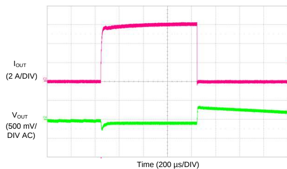
Figure 26. LM73606 5-V 400-kHz Load Transient V_{IN} = 12\text{ V} , I_{OUT} = 10\text{ mA} to 6 A to 10 mA
