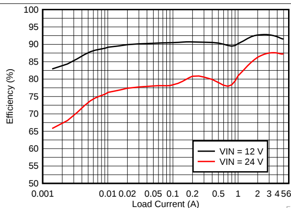
Figure 10. LM73605 5-V 2.2-MHz Efficiency in Auto Mode
