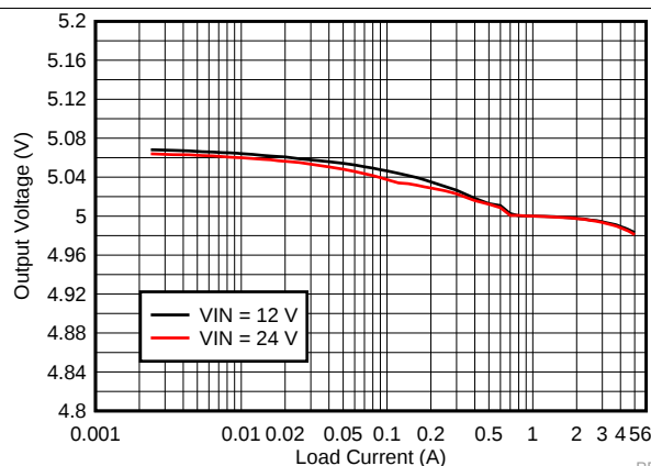
Figure 12. LM73605 5-V 2.2-MHz V_{OUT} Regulation in Auto Mode
