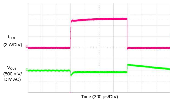
Figure 14. LM73605 5-V 2.2-MHz Load Transient V_{IN} = 12\text{ V} , I_{OUT} = 10\text{ mA to } 5\text{ A to } 10\text{ mA}
