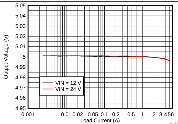
Figure 19. LM73605 5-V 400-kHz V_{OUT} Regulation in FPWM Mode
