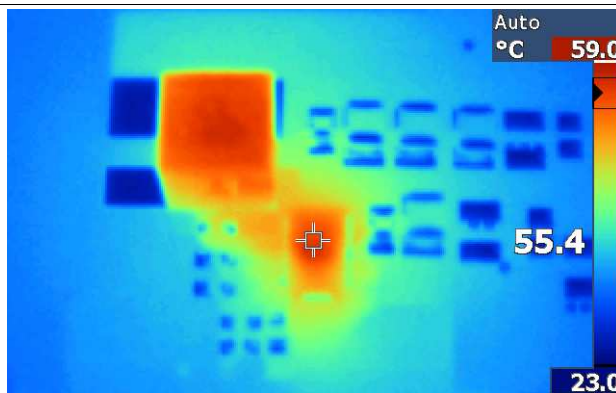
Figure 27. LM73605 5-V 400-kHz EVM Thermal Picture with V_{IN} = 12\text{ V} I_{OUT} = 6\text{ A}
