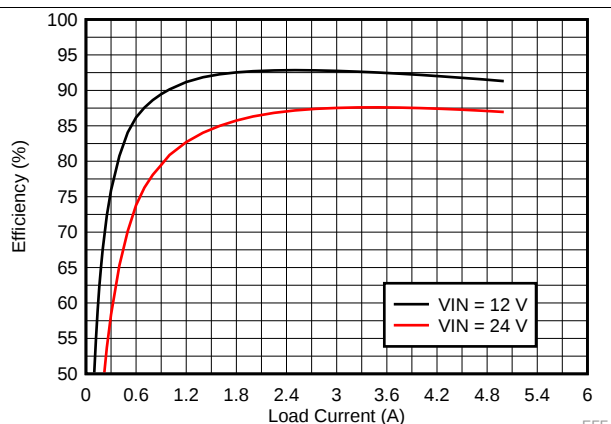
Figure 11. LM73605 5-V 2.2-MHz Efficiency in FPWM Mode
