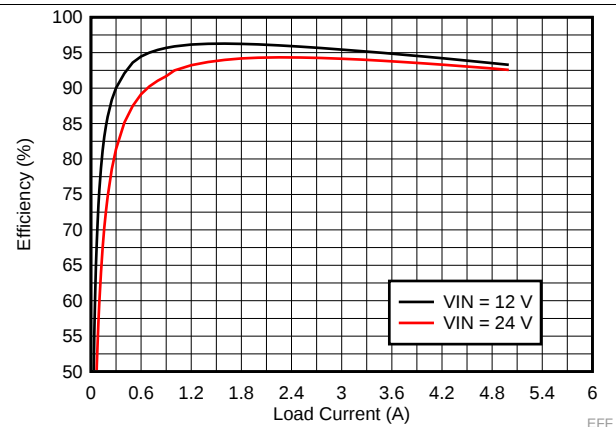
Figure 17. LM73605 5-V 400-kHz Efficiency in FPWM Mode
