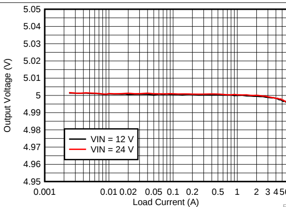
Figure 25. LM73606 5-V 400-kHz V_{OUT} Regulation in FPWM Mode
