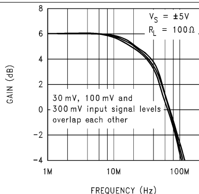
Figure 39. Closed Loop Frequency Response vs. Input Signal Level ( A_V = +2 )
