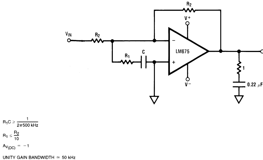
Figure 13. Inverting Unity Gain Operation
