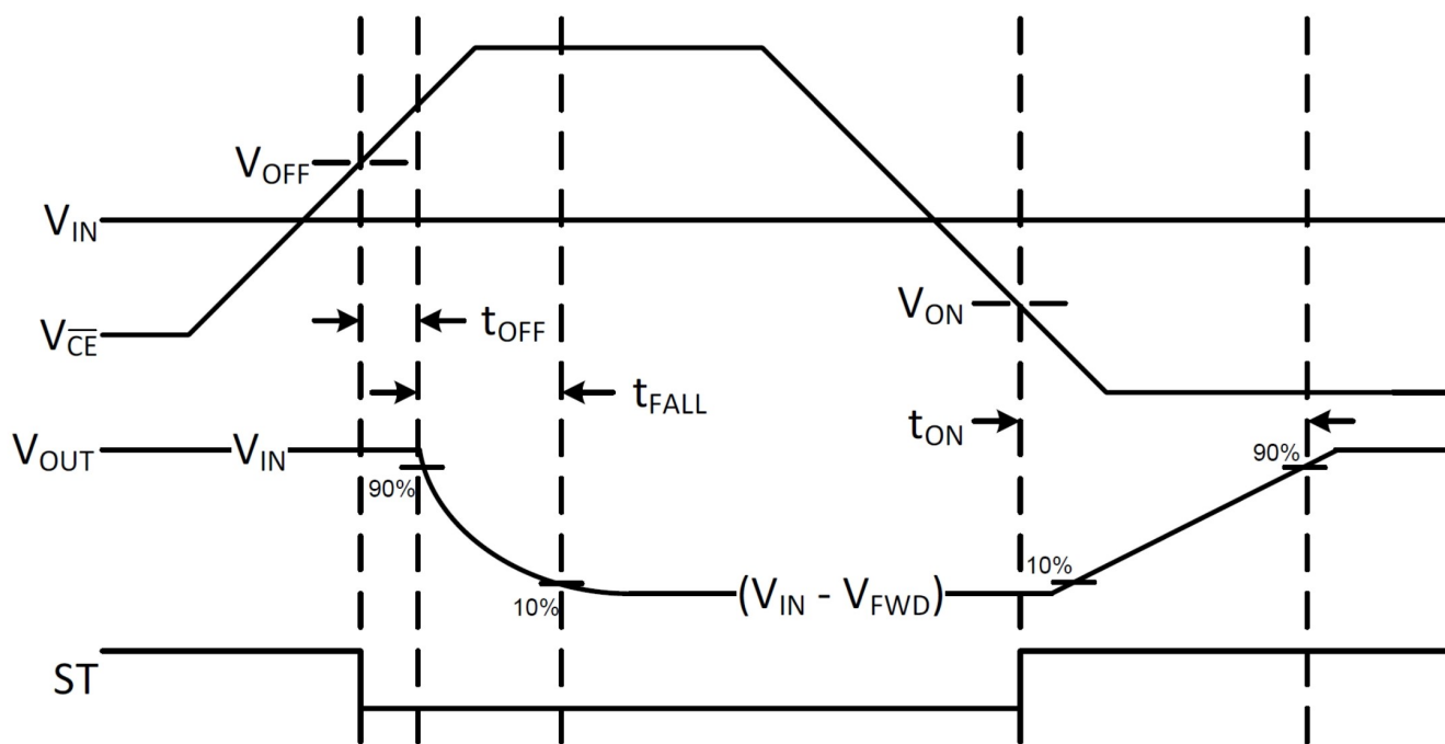
Figure 11. Timing Diagram
