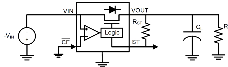
Figure 12. RPP Protection Circuit
