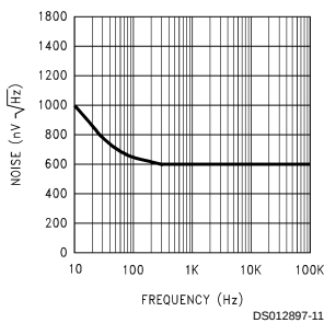
Noise Voltage
