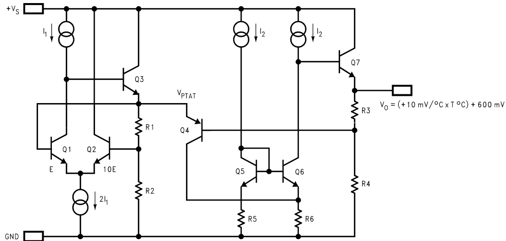
FIGURE 6. Simplified Schematic
