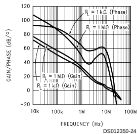
Open Loop Gain/ Phase ( V_S = 5V )
