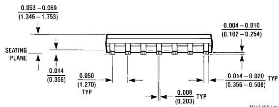
14-Lead (0.150") Molded Small Outline Package, JEDEC Order Number LM6154ACM or LM6154BCM NSC Package Number M14A
