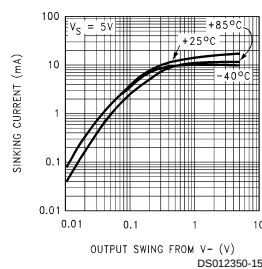
Output Voltage vs. Sink Current
