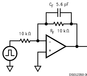
FIGURE 1. Typical Inverting Gain Circuit A_V = -1
