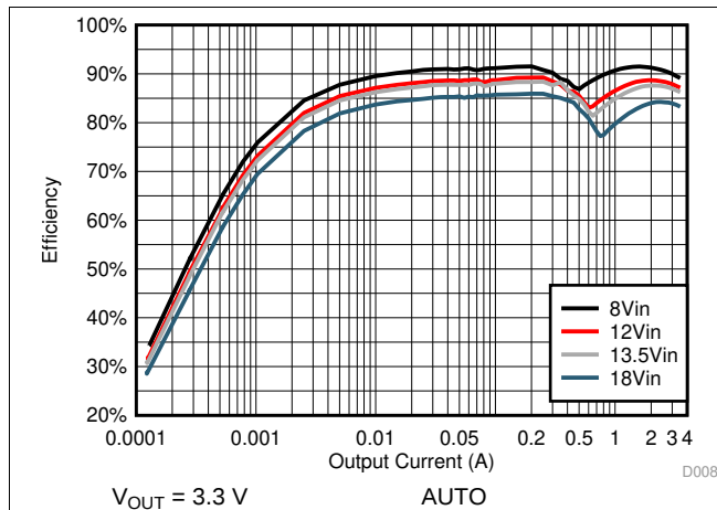
Figure 39. Efficiency
