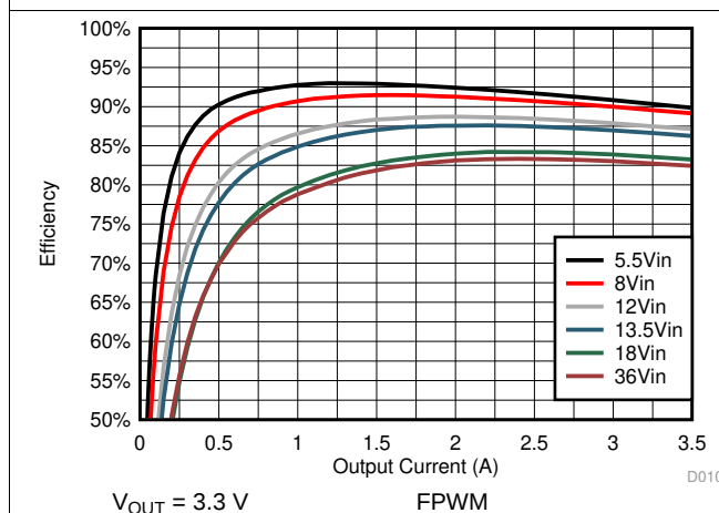
Figure 41. Efficiency
