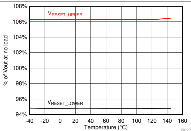
Figure 8. RESET Threshold as Percentage of Output Voltage
