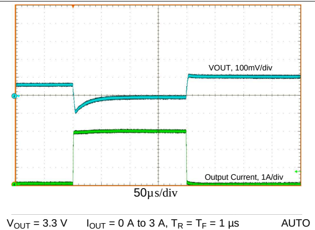
Figure 42. Load Transient
