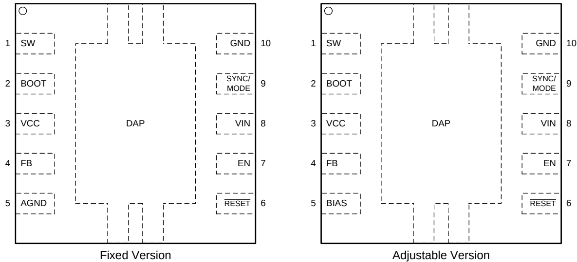
Pin Functions
