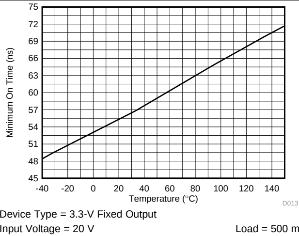
Figure 1. Minimum On-Time vs Temperature
