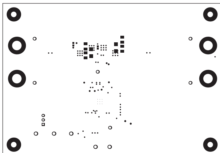
Figure 19. Bottom Solder
