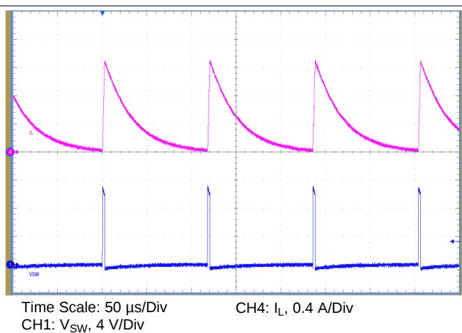
Figure 83. Short Circuit
