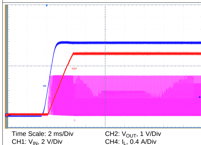
Figure 82. Full-Load Start-Up
