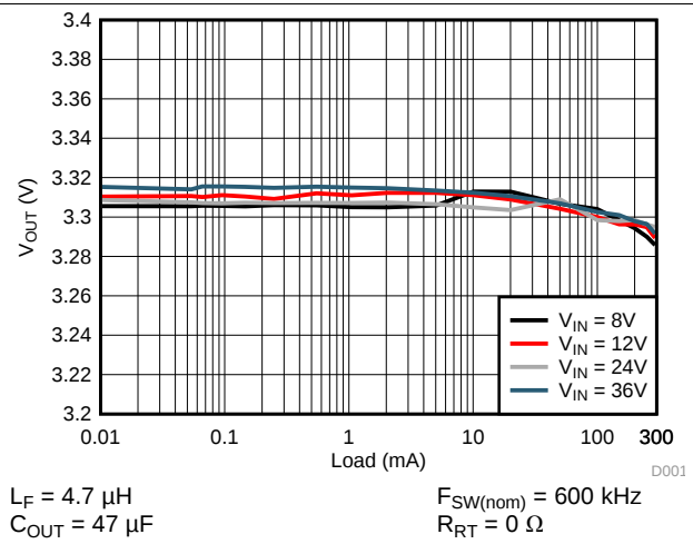
Figure 72. Converter Regulation
