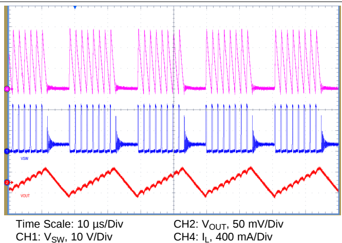
Figure 74. Full-Load Switching Waveforms, V_{IN} = 24\ \text{V}
