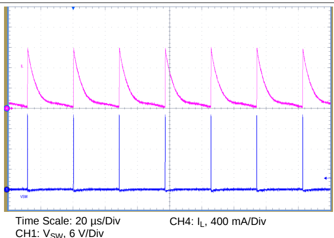
Figure 76. Short Circuit, V_{IN} = 24\ \text{V}
