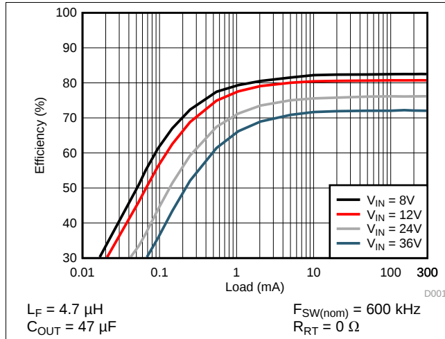
Figure 71. Converter Efficiency
