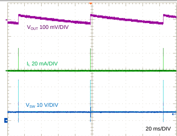
5-V, 25-mA Design
