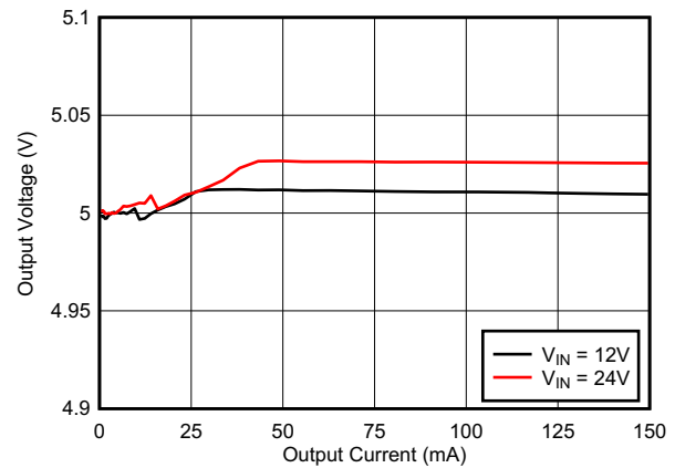
Figure 39. Load Regulation
