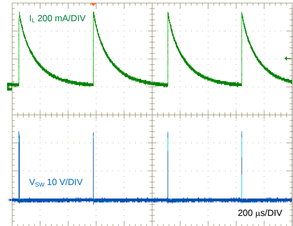
5-V, 150-mA Design
