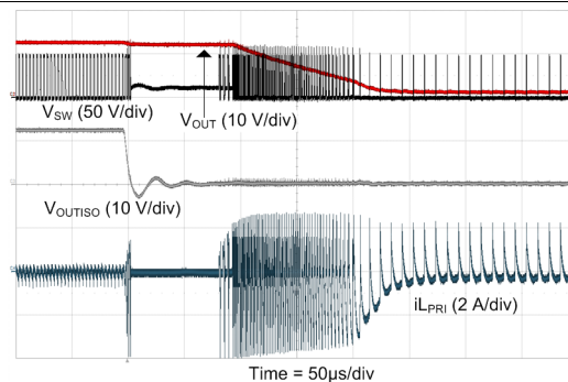
Figure 40. Secondary-Side Short at I_{OUT2} = 0 A and I_{PR1} = 0 A
