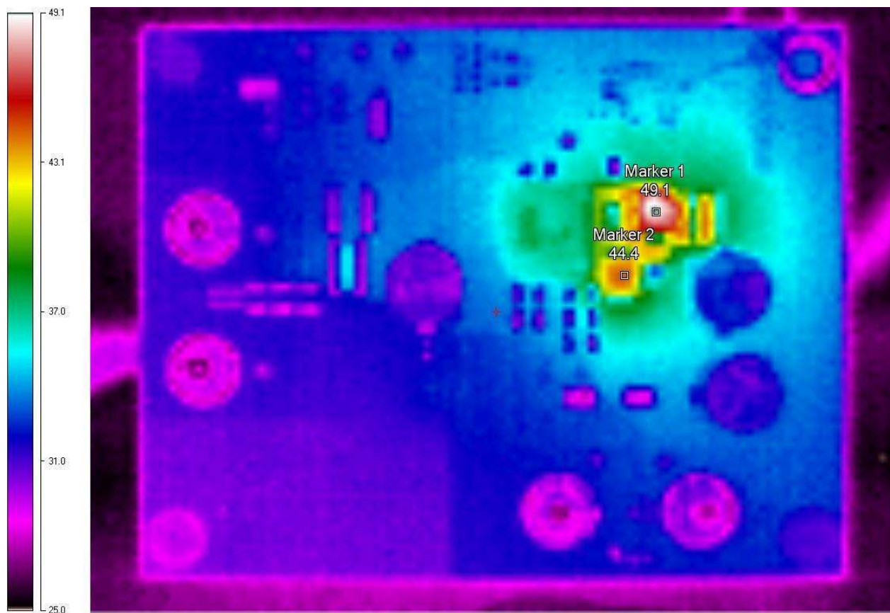
Figure 6. Thermal Image V_{IN} = 6\text{ V} I_{OUT} = 2\text{ A} , No forced air cooling
