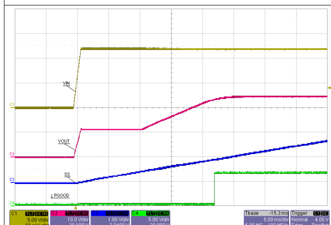
Figure 13. Start-Up, V_{IN} = 12\text{ V} , I_{OUT} = 2\text{ A}
