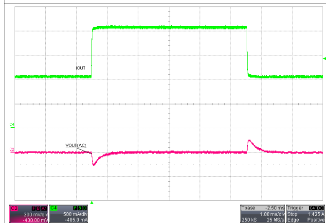
Figure 17. Load Transient, V_{IN} = 12\text{ V} , I_{OUT} = 1\text{ A to }2\text{ A}
