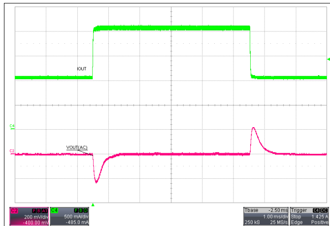
Figure 15. Load Transient, V_{IN} = 6\text{ V} , I_{OUT} = 1\text{ A to }2\text{ A}
