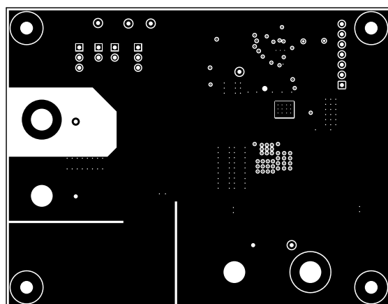
Figure 25. Signal Layer 1
