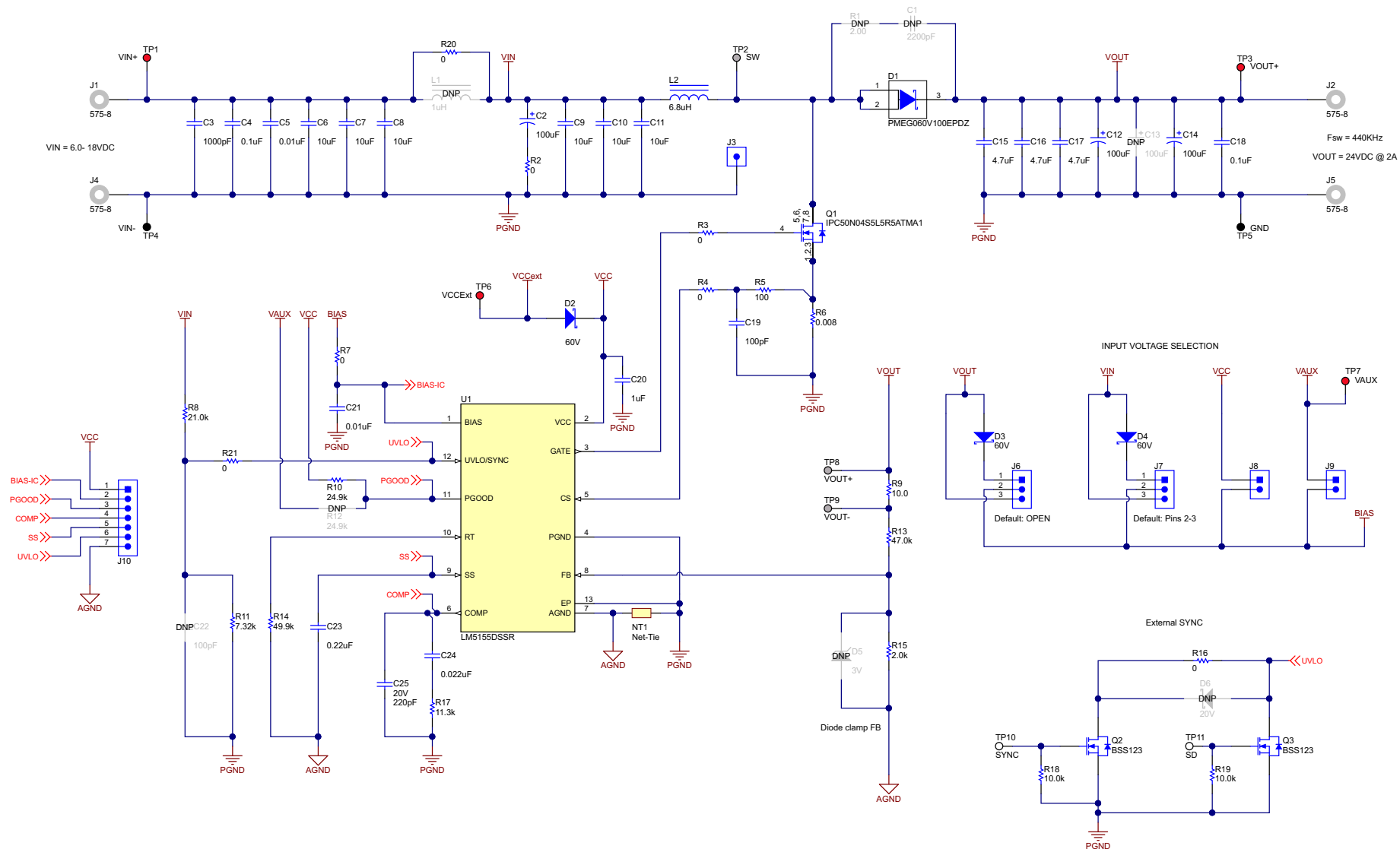
Figure 29. LM5155EVM-BST Schematic
