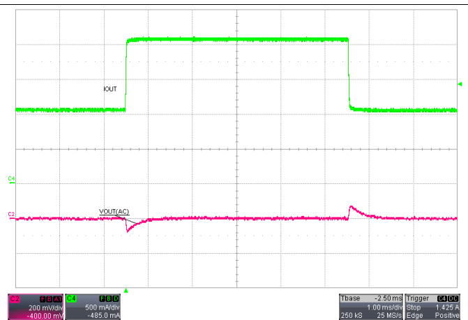
Figure 18. Load Transient, V_{IN} = 18\text{ V} , I_{OUT} = 1\text{ A to }2\text{ A}
