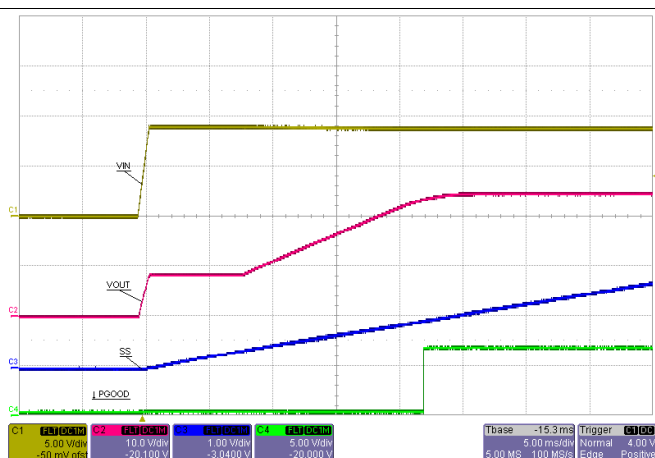
Figure 12. Start-Up, V_{IN} = 9\text{ V} , I_{OUT} = 2\text{ A}
