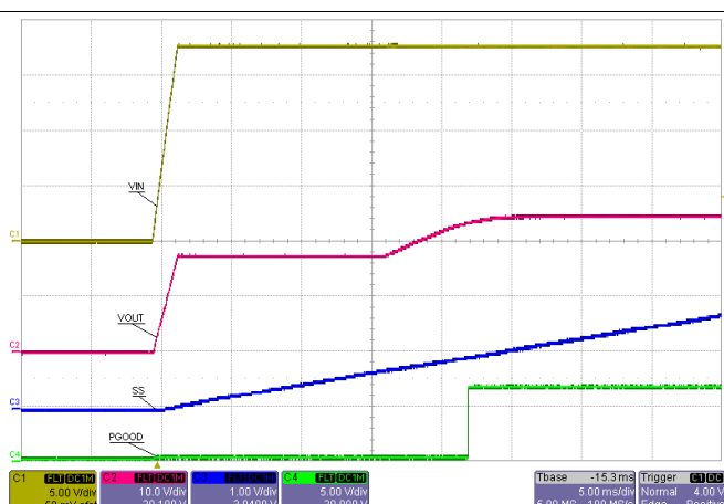
Figure 14. Start-Up, V_{IN} = 18\text{ V} , I_{OUT} = 2\text{ A}
