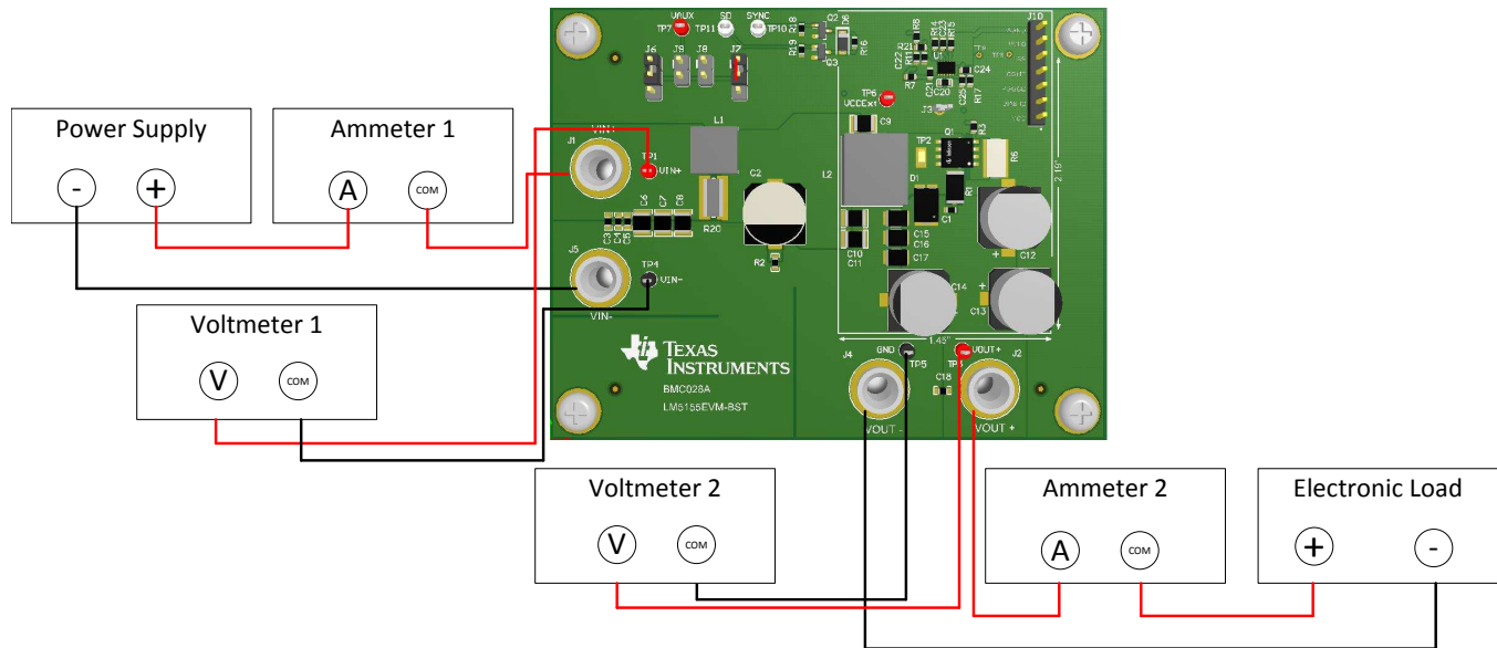
Figure 3. Test Setup
