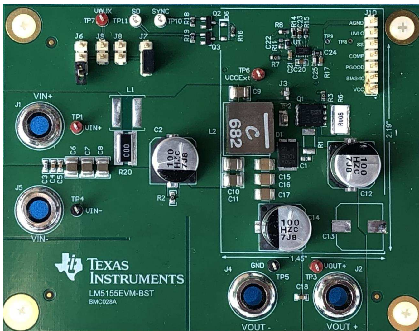
Figure 2. EVM Photo
