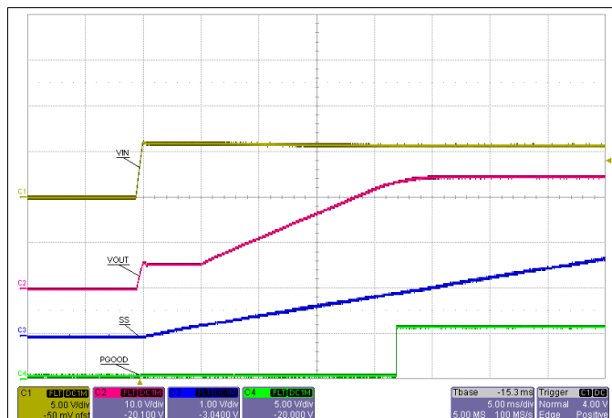
Figure 11. Start-Up, V_{IN} = 6\text{ V} , I_{OUT} = 2\text{ A}
