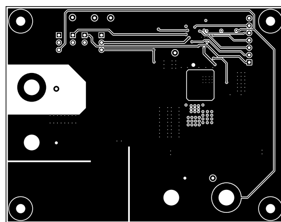
Figure 26. Signal Layer 2
