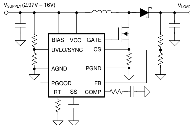
Figure 21. 2.97-V Start-Up (BIAS = VCC)
