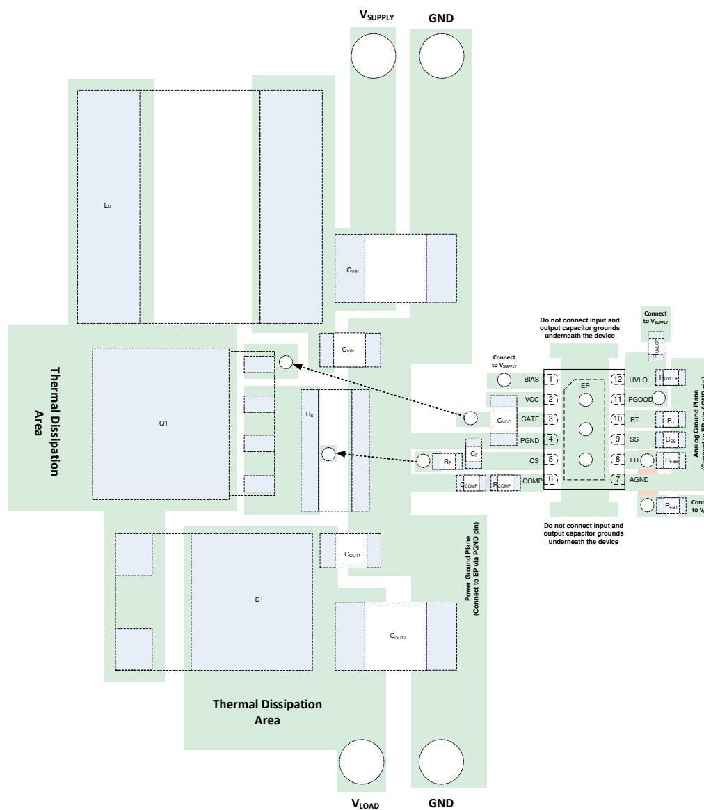
Figure 51. PCB Layout Example 1
