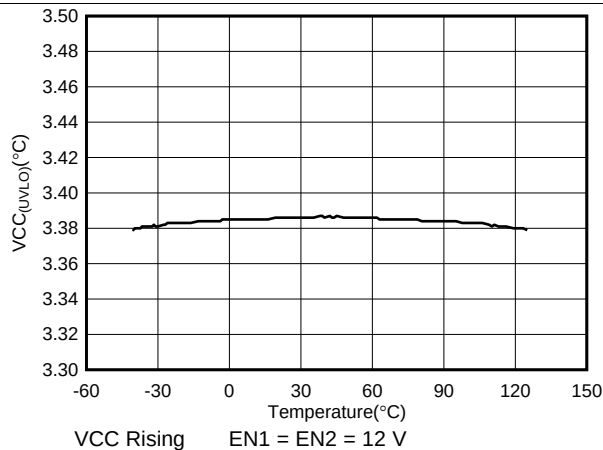
Figure 6. V_{\text{CC(UVLO)}} vs Temperature
