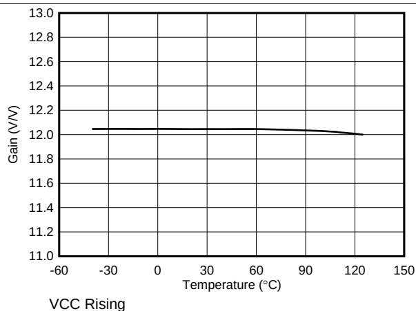
Figure 12. Current Sense Amplifier Gain vs Temperature
