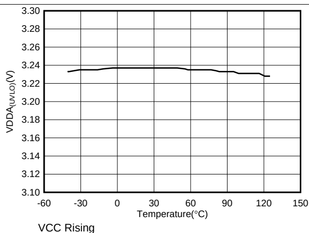
Figure 8. V_{DDA(UVLO)} vs Temperature
