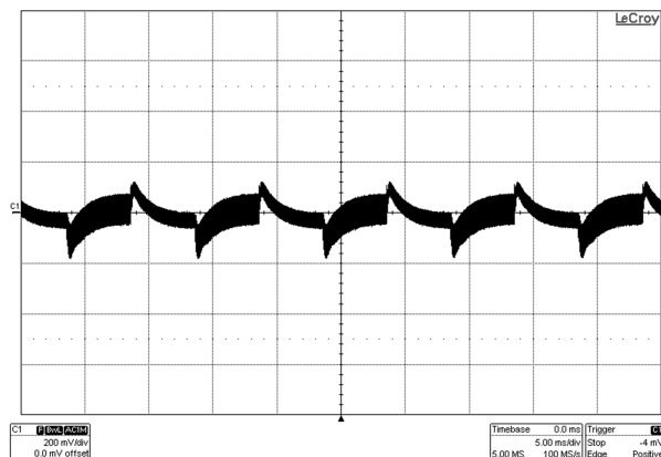
Figure 3. Load Transient
