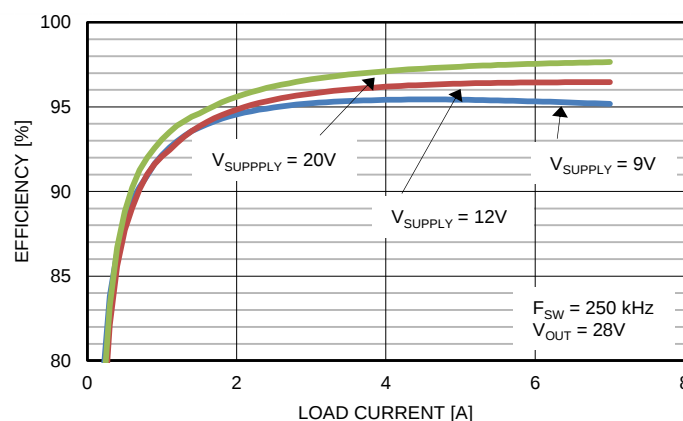
Figure 2. Efficiency
