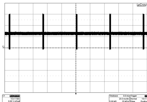
Figure 6. Skip Cycle
