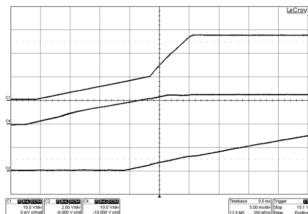
Figure 8. Startup
