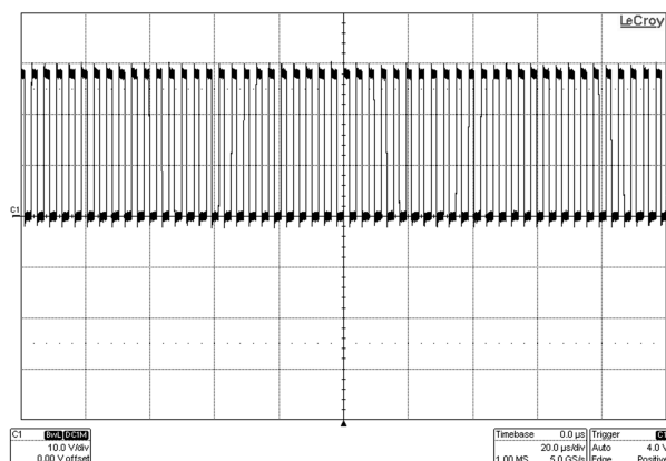
Figure 7. Forced PWM
