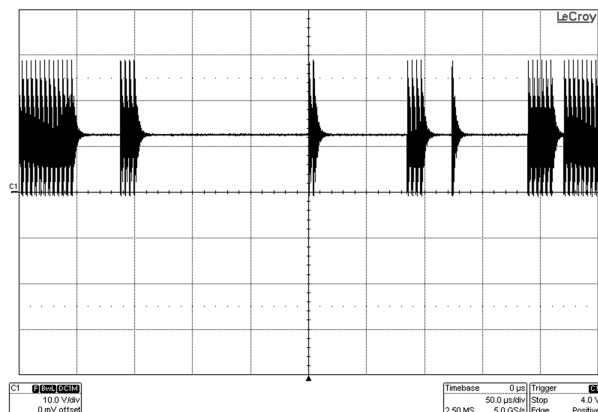
Figure 5. Pulse Skip
