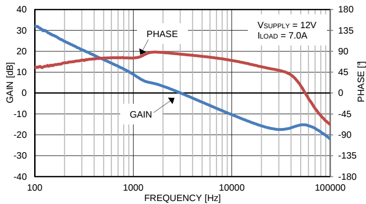
Figure 9. Loop Response
