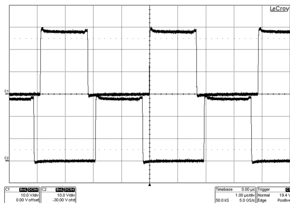
Figure 4. Interleaving
