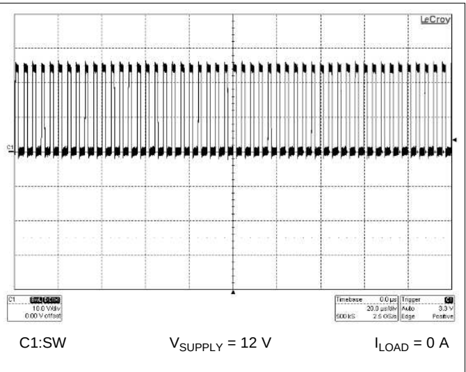
Figure 44. Forced PWM
