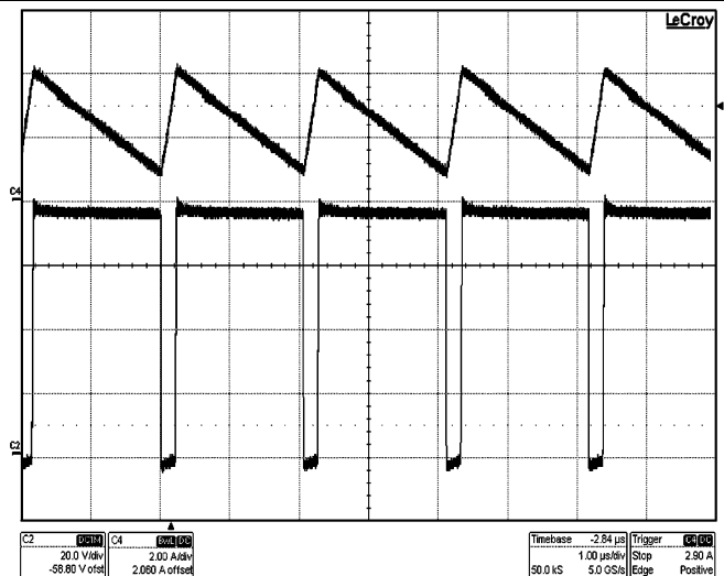
Figure 24. Switching Node Voltage V_{IN} = 24 V, Load Current = 2 A
