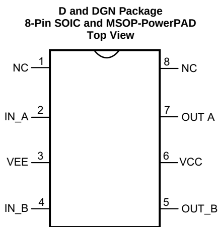
Pin Functions
