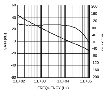
Figure 26. Overall Loop Gain and Phase
