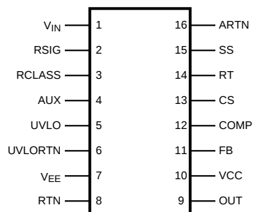
Figure 2. 16 Lead TSSOP
