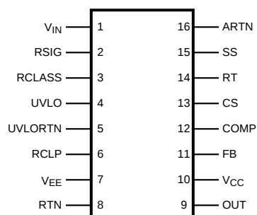
Figure 2. 16 Lead TSSOP/WSO See Package Number PW or NHQ0016A
