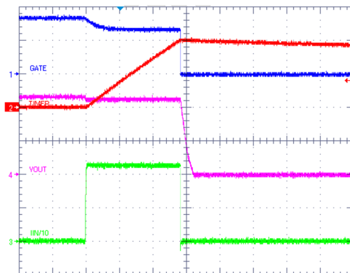
Figure 8. Fault Timeout
