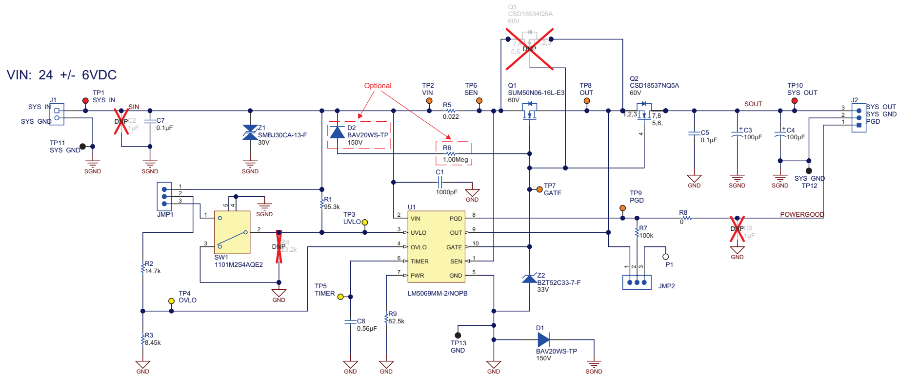
Figure 18. LM5069EVM-627 Schematic
