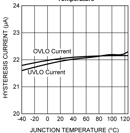
UVLO & OVLO Hysteresis Current vs. Temperature
