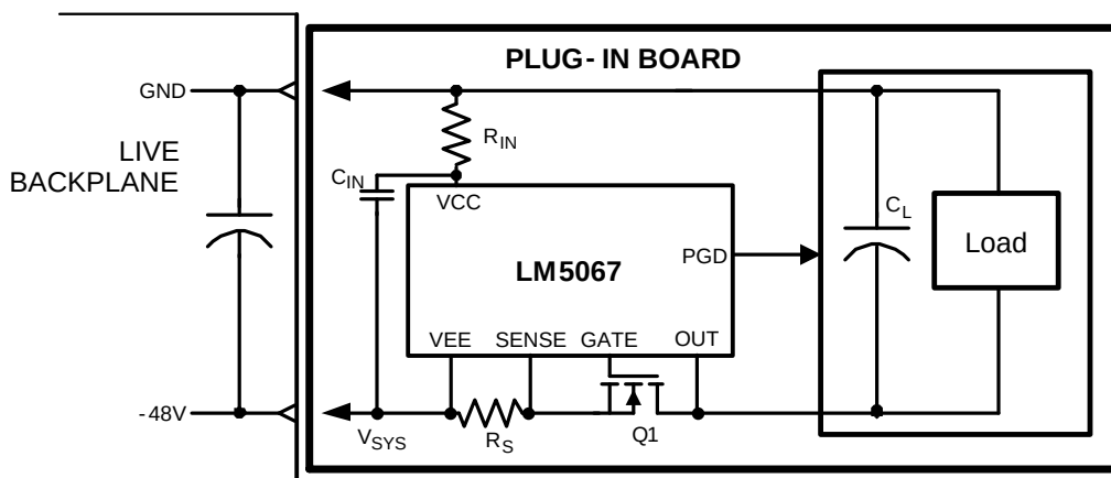
Figure 5. LM5067 Application
