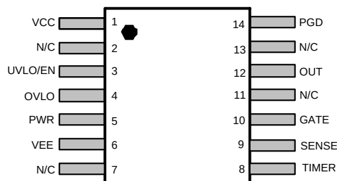
Figure 3. Top View 14-Lead SOIC
