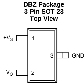
Pin Functions
