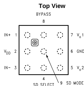
Figure 3. 9 Bump DSBGA Package See Package Number YZR0009AAA
