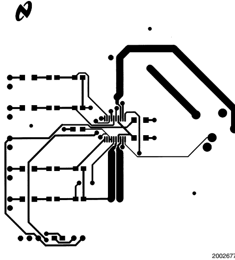
FIGURE 20. Recommended MT PC Board Layout: Component-Side Layout
