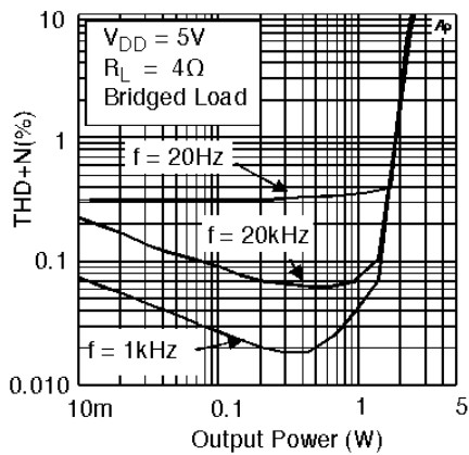
LM4868MTE THD+N vs Output Power
