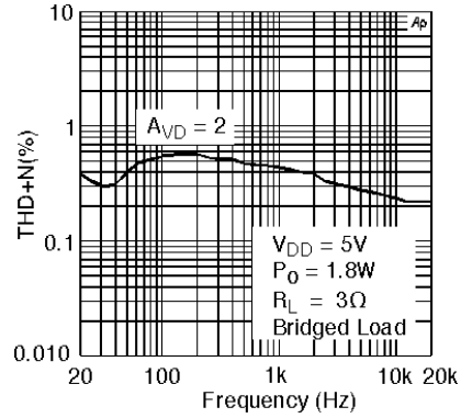
LM4868MTE THD+N vs Frequency
