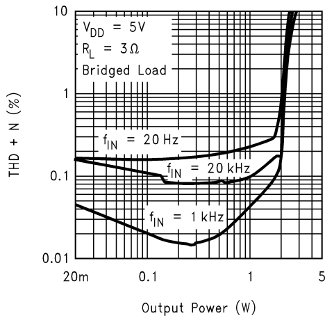
LM4868LQ THD+N vs Output Power
