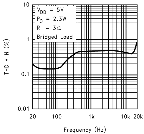
LM4868LQ THD+N vs Frequency
