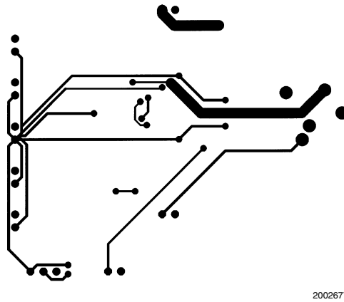
FIGURE 21. Recommended MT PC Board Layout: Bottom-Side Layout
