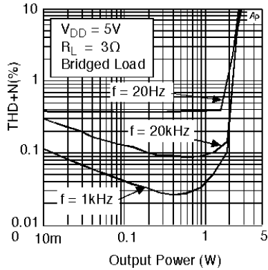
LM4868MTE THD+N vs Output Power
