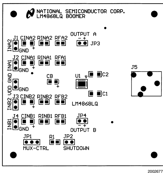
FIGURE 9. Recommended LQ PC Board Layout: Component-Side Silkscreen
