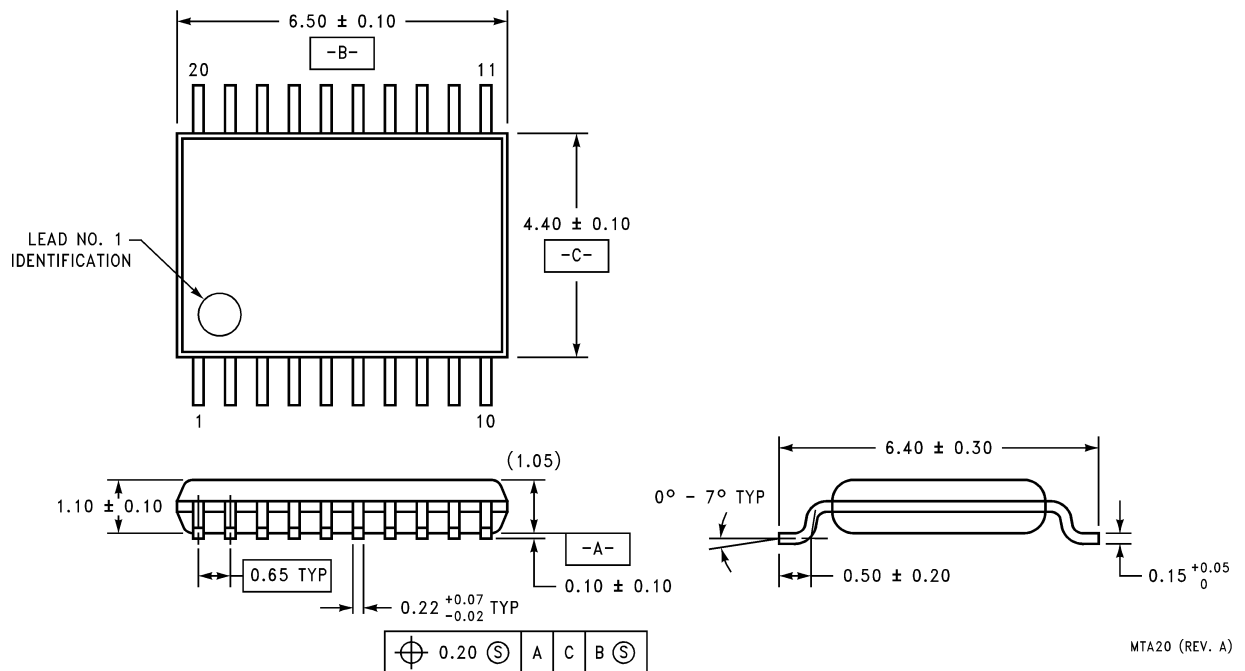
20-Lead MOLDED PKG, TSSOP, JEDEC, 4.4mm BODY WIDTH Order Number LM4868MT NS Package Number MTC20
