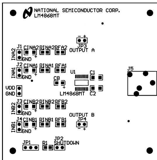
FIGURE 19. Recommended MT PC Board Layout: Component-Side Silkscreen
