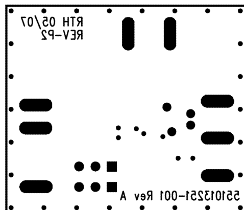
Figure 39. Bottom Silkscreen
