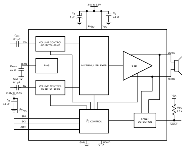
Typical Audio Amplifier Application Circuit
