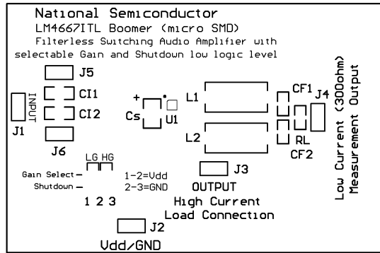
Silk Screen
