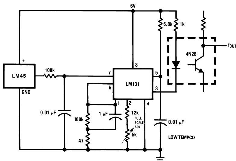
Figure 26. LM45 With Voltage-To-Frequency Converter And Isolated Output ( 2.5^\circ C to +100^\circ C ; 25 Hz to 1000 Hz)
