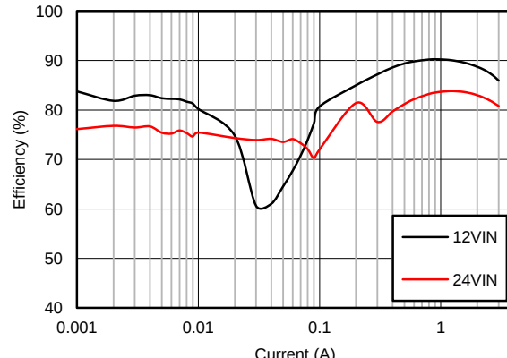
Figure 80. Efficiency
