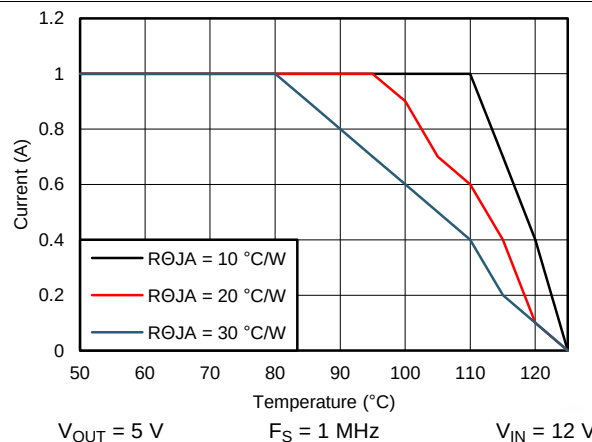
Figure 76. Derating Curve
