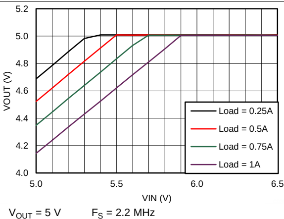
Figure 17. Dropout Curve
