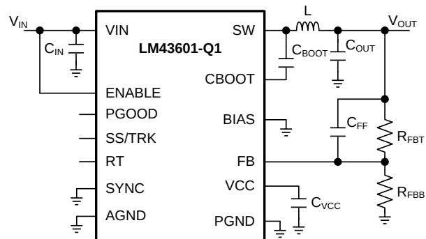
Figure 45. LM43601-Q1 Basic Schematic for V_{OUT} < 3.3 V, Tie BIAS to Ground
