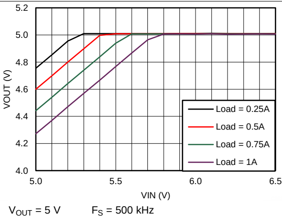
Figure 15. Dropout Curve
